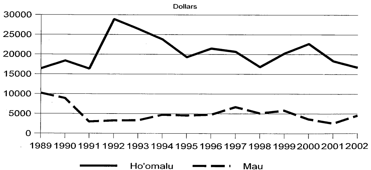
FIGURE 3-15: Inflation-adjusted Gross Revenue per Trip of Vessels Bottomfish Fishing in the Mau Zone and Ho'omalulu Zone, 1989-2002
