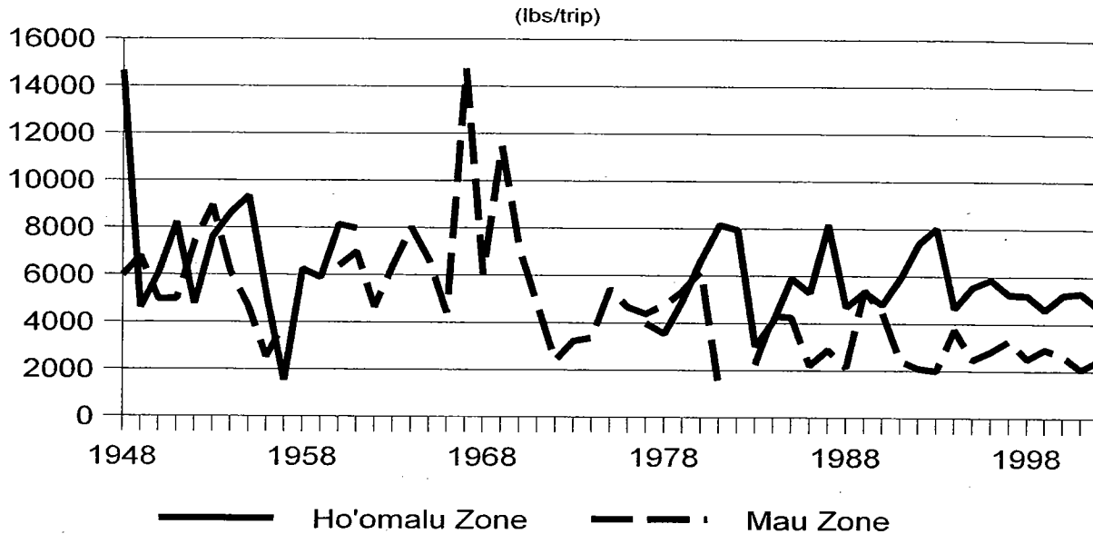
FIGURE 3-10: Catch Per Unit Effort of Vessels Fishing in the Mau Zone and Ho'omaluu Zone, 1948-2002 (HDAR Data)
