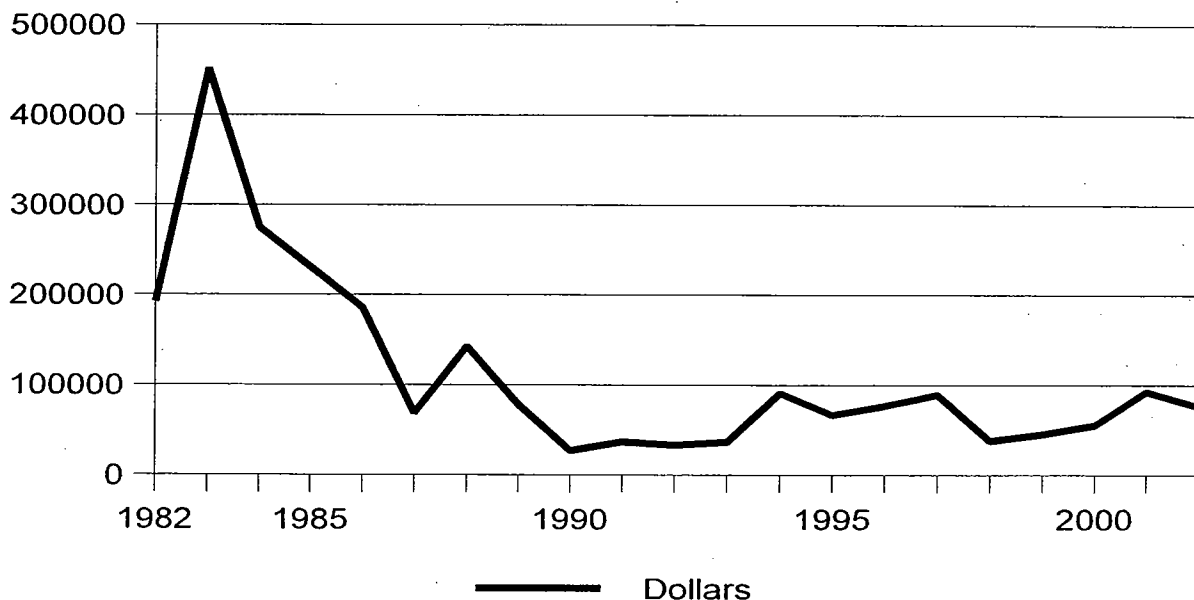
FIGURE 3-18: Inflation-adjusted Gross Revenue in the American Samoa Bottomfish Fishery, 1982-2002
