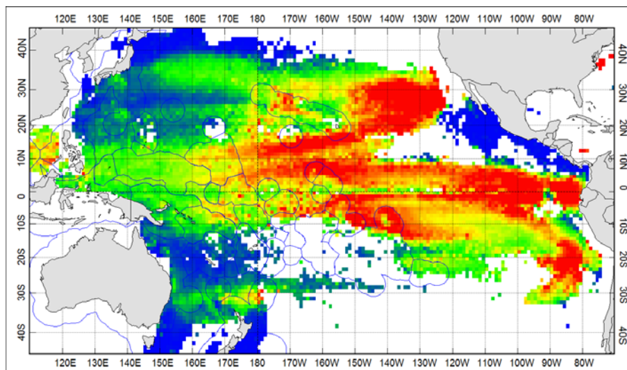
Figure 3. Pacific-wide longline CPUE (Japan), aggregated data (1966-2006). CPUE ranges from Blue (lower) to Red (higher) areas of CPUE
