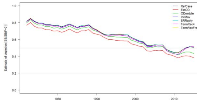
Figure SKJ 7. Estimated fisheries depletion S_{B}/S_{BF=0} , for each of the sensitivity models.
