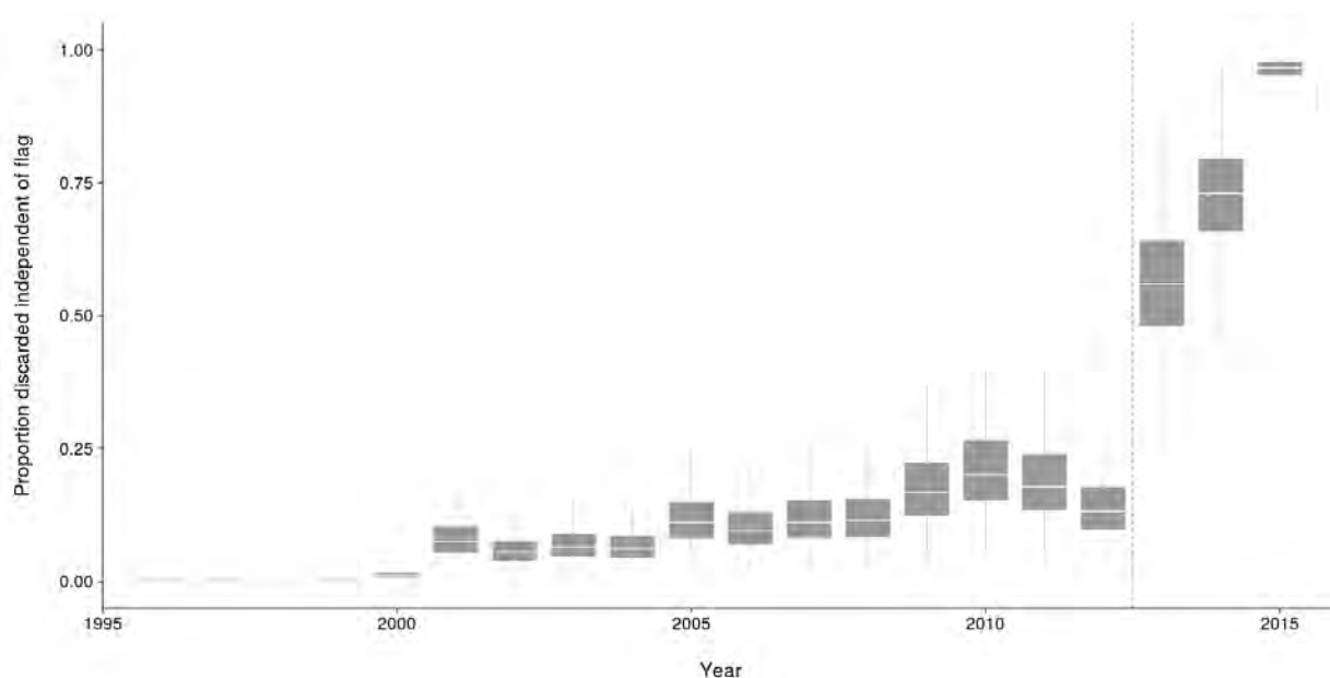
Figure 9: Year effects, independent of flag, estimated for the proportion of individuals discarded by year in the binomial model predicting discard rates over time. The white line shows the median and the box outlines the inter - quartile range.
