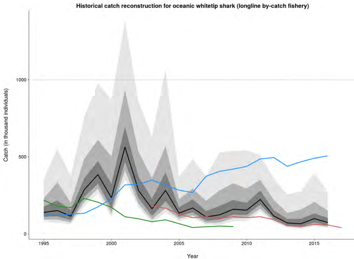
Figure 5: Median predictions of oceanic whitetip shark catch in the WCPO for the longline by-catch fleet based on a model of longline observed catch rates applied to LBEST effort. The light, dark and darker grey bounds show the 0.025 th -0.975 th , 0.10 th -0.90 th and 0.25 th -0.75 th uncertainty bounds. For comparison with our estimates, the blue line shows the median prediction of historical catch based on global fin trade statistics, the red line shows the prediction of historical catch published in (Peatman et al. 2018), and the green line shows the historical catches used for this fleet in the reference case for the 2012 assessment.
