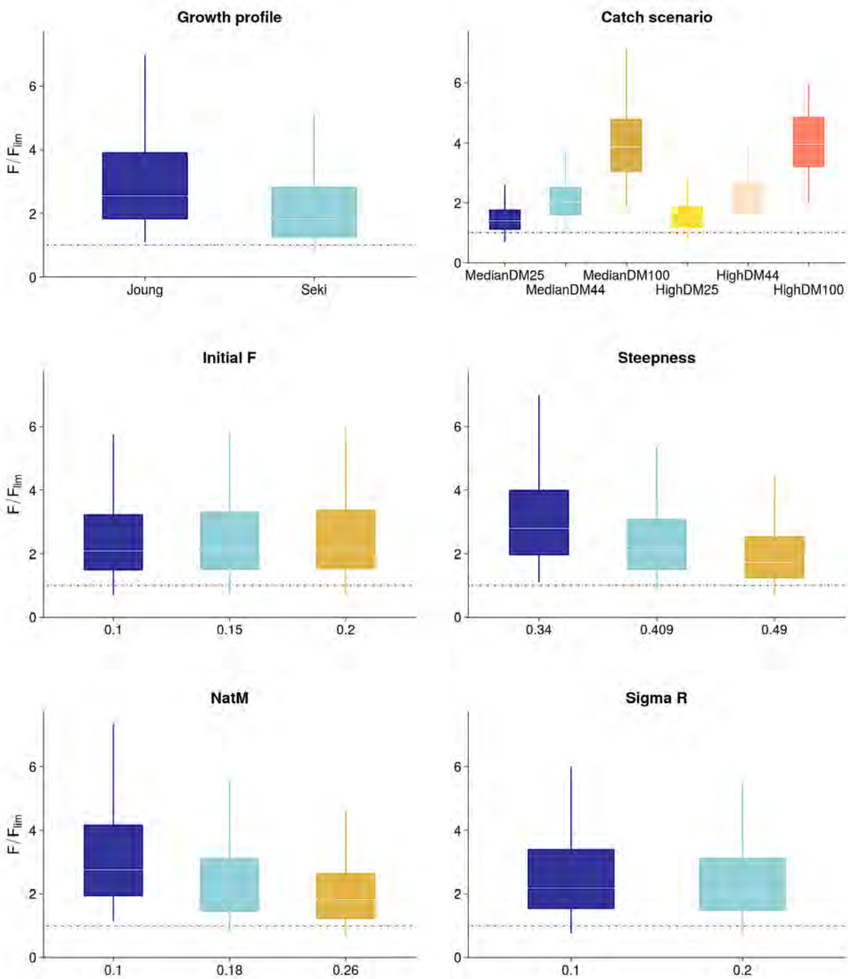
Figure 35: Median (white bar) and inter - quartile bounds (box) for F/F_{lim} in the final year of the assessment for each structural uncertainty axis. The whiskers extend to 1.5 \times the interquartile range.
