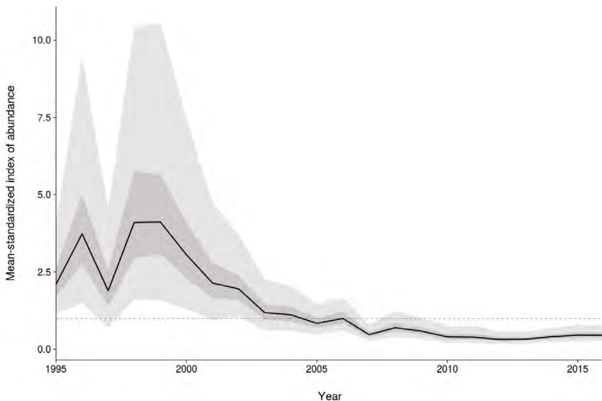
Figure 13: Mean - standardized CPUE index used in this assessment of oceanic whitetip shark. The light and dark grey bounds show the 0.025 th - 0.975 th and 0.25 th - 0.75 th uncertainty bounds around the year effects. The dashed line at 1 shows the reference mean value.
