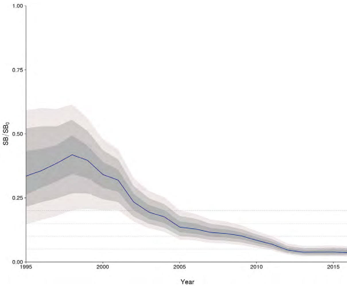
Figure 30: Median prediction of depletion in spawning biomass over all (unweighted) grid runs, with 0.025 th - 0.975 th , 0.10 th - 0.90 th and 0.25 th - 0.75 th quantile intervals. The horizontal grey lines are placed at intervals of 5% in the lower part of the graph to aid visualization.
