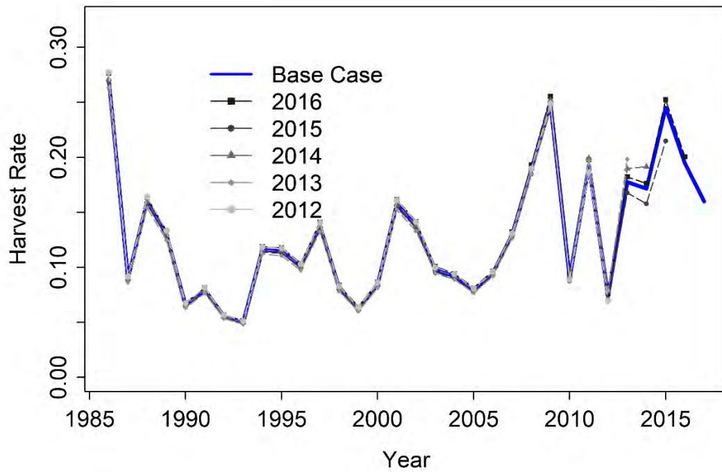
Figure 42. Retrospective analysis for biomass (top) and harvest rate (bottom) with the base case model ending in 2017 as a reference (blue line) and with terminal year set as 2016 through 2012 (gray lines) for bottomfish management unit species in American Samoa.
