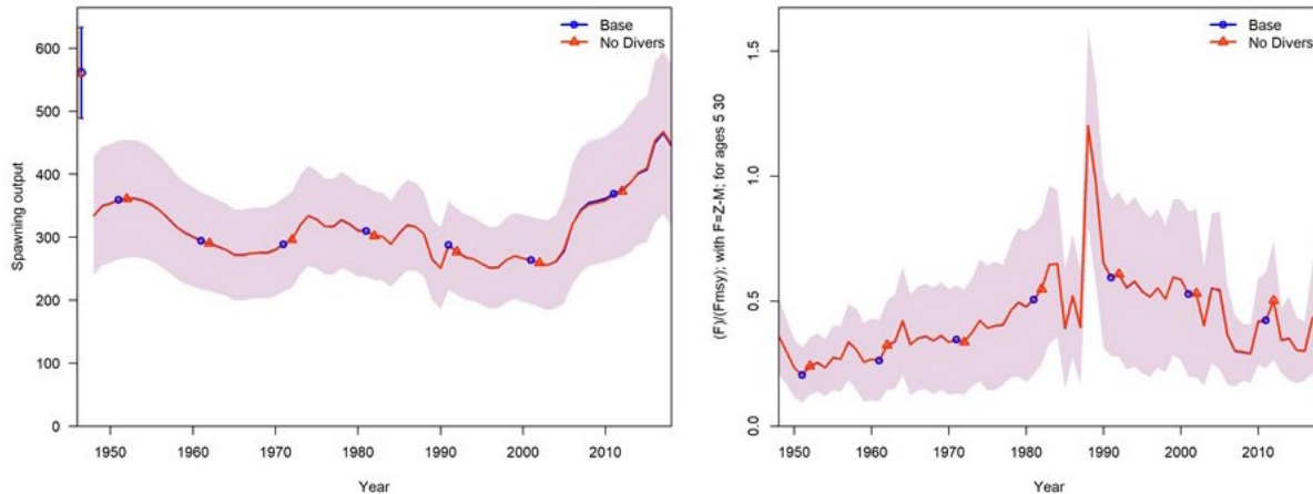
Figure 3. A comparison of model outputs (SSB and F/FMSY) for the base case and a sensitivity run that did not include the fishery-independent diver survey index.
