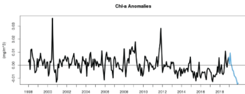
Monthly Anomaly 1998-2018 2019
