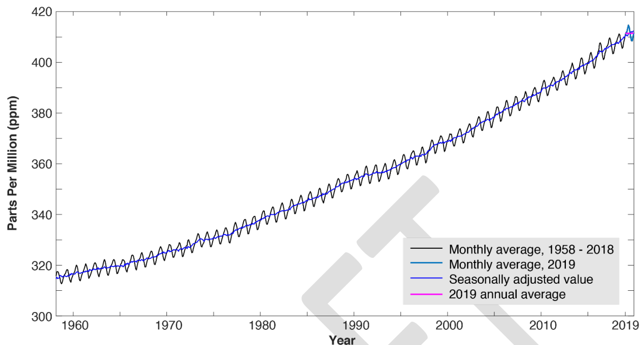
Figure 5. Monthly mean (black) and seasonally corrected (blue) atmospheric carbon dioxide at Mauna Loa Observatory, Hawaii
