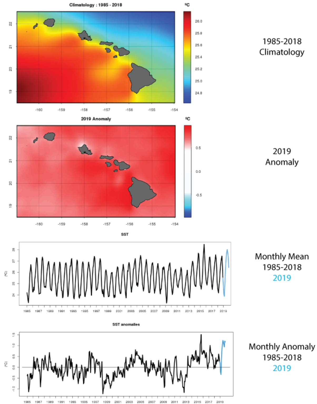
Figure 11. Sea surface temperature climatology and anomalies from 1985-2019
