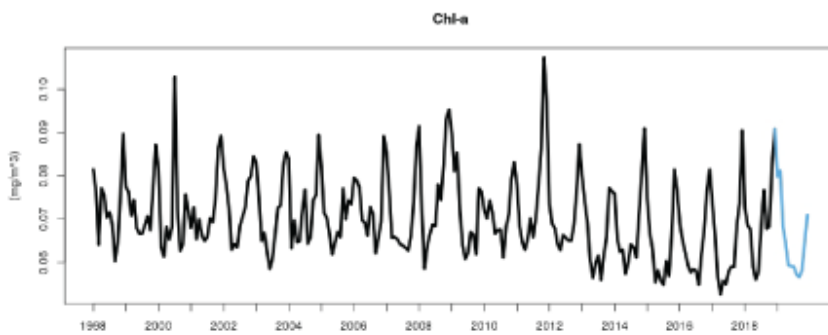
Monthly Mean 1998-2018 2019
