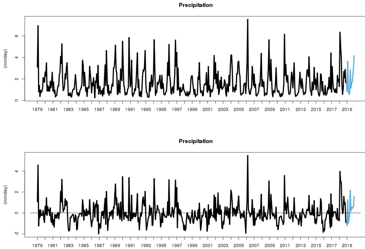
Figure 14. CMAP precipitation across the MHI Grid with 2019 values in blue
