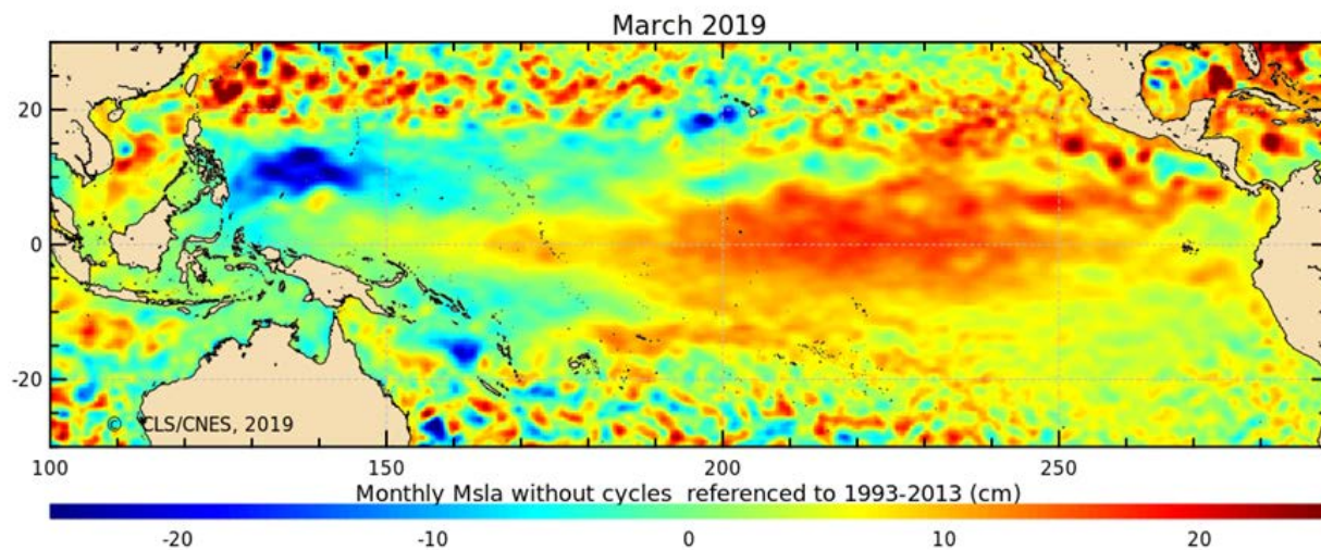
Figure 15a. Sea surface height and anomaly
