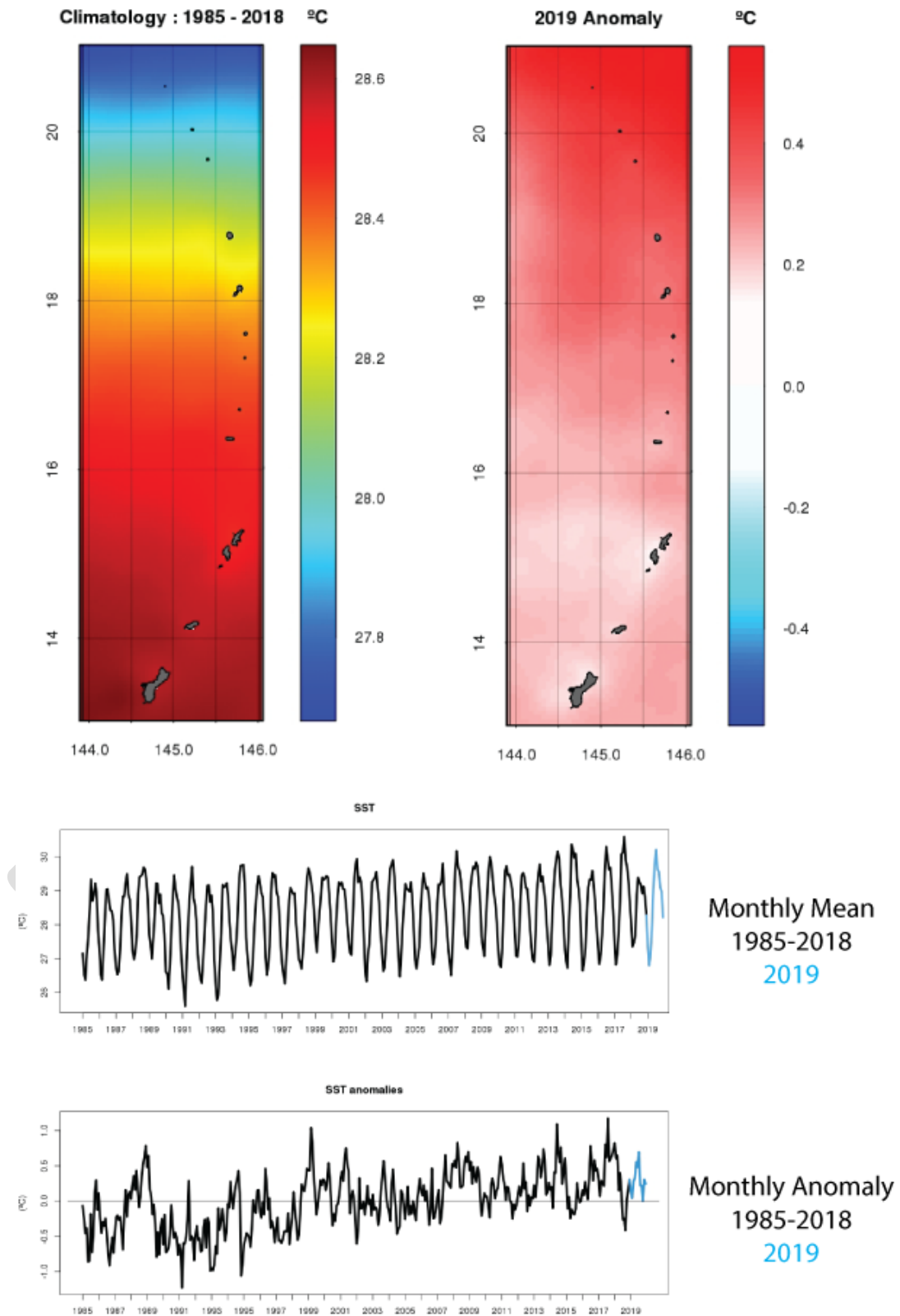
Figure 11. Sea surface temperature climatology and anomalies from 1985-2019
