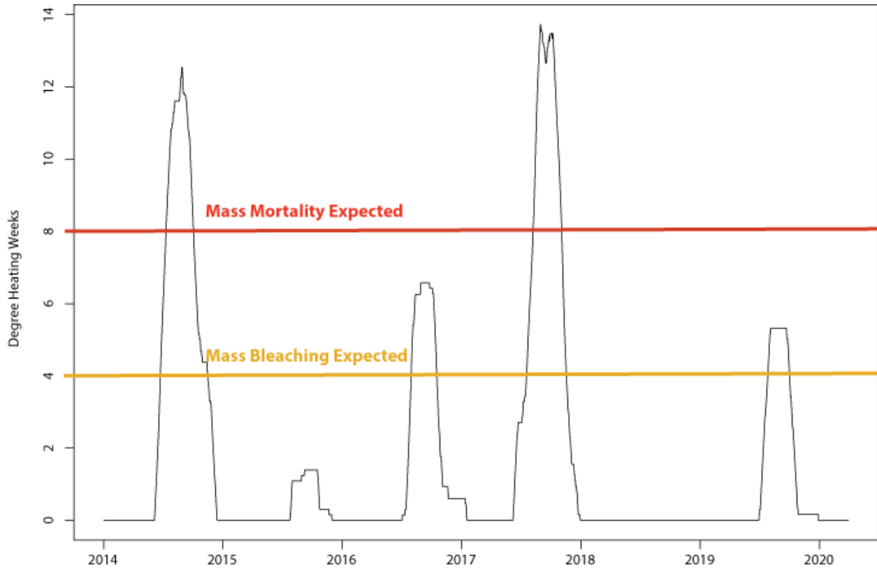
Figure 12. Coral Thermal Stress Exposure measured at CNMI Virtual Station 2014-2019 (Coral Reef Watch Degree Heating Weeks)
