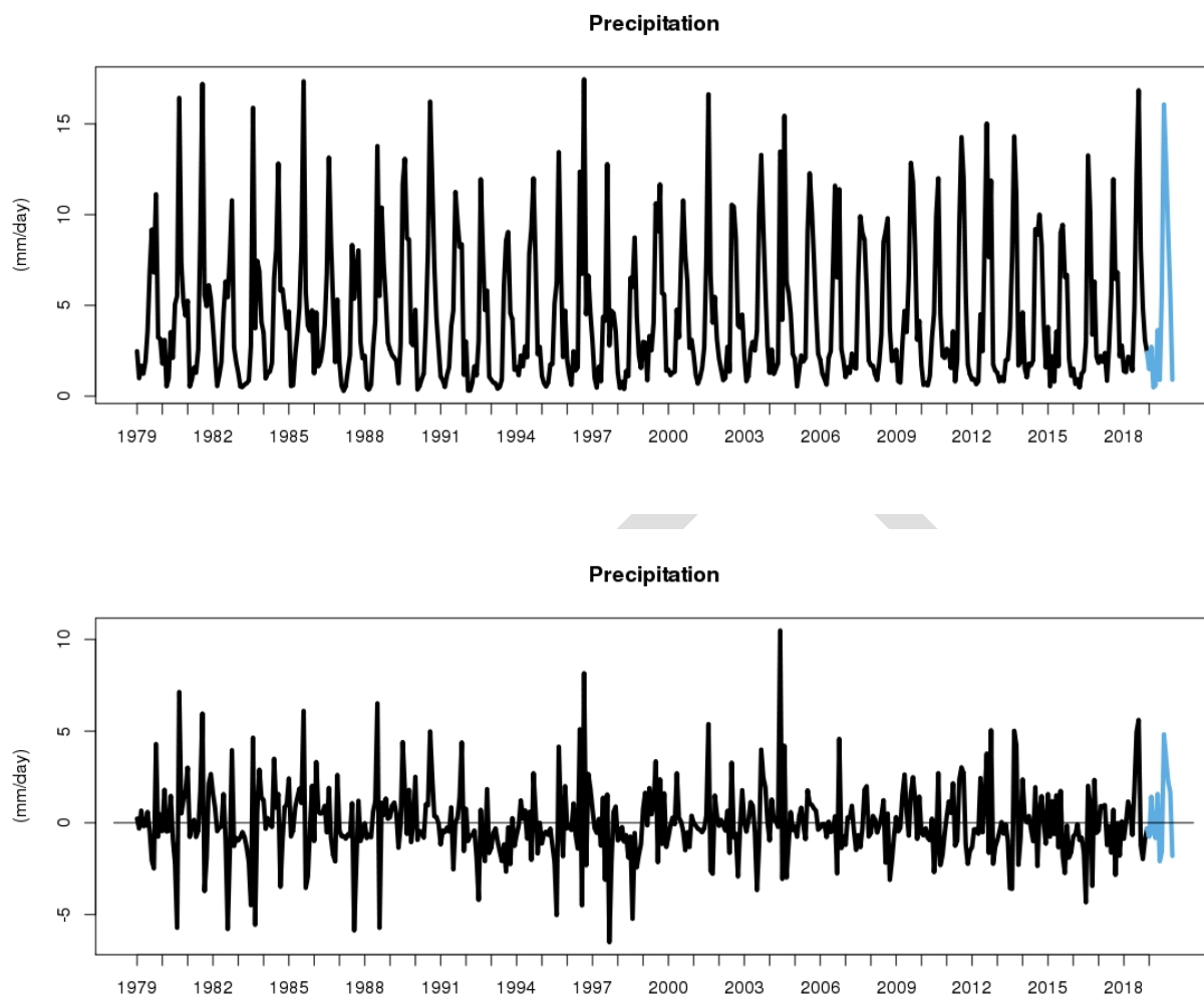
Figure 14. CMAP precipitation across the Marianas Grid with 2019 values in blue
