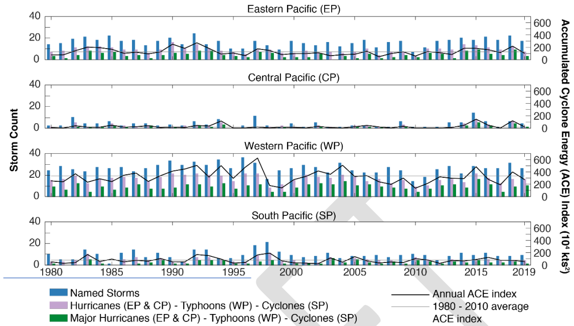
Figure 10. 2019 tropical storm totals by region
