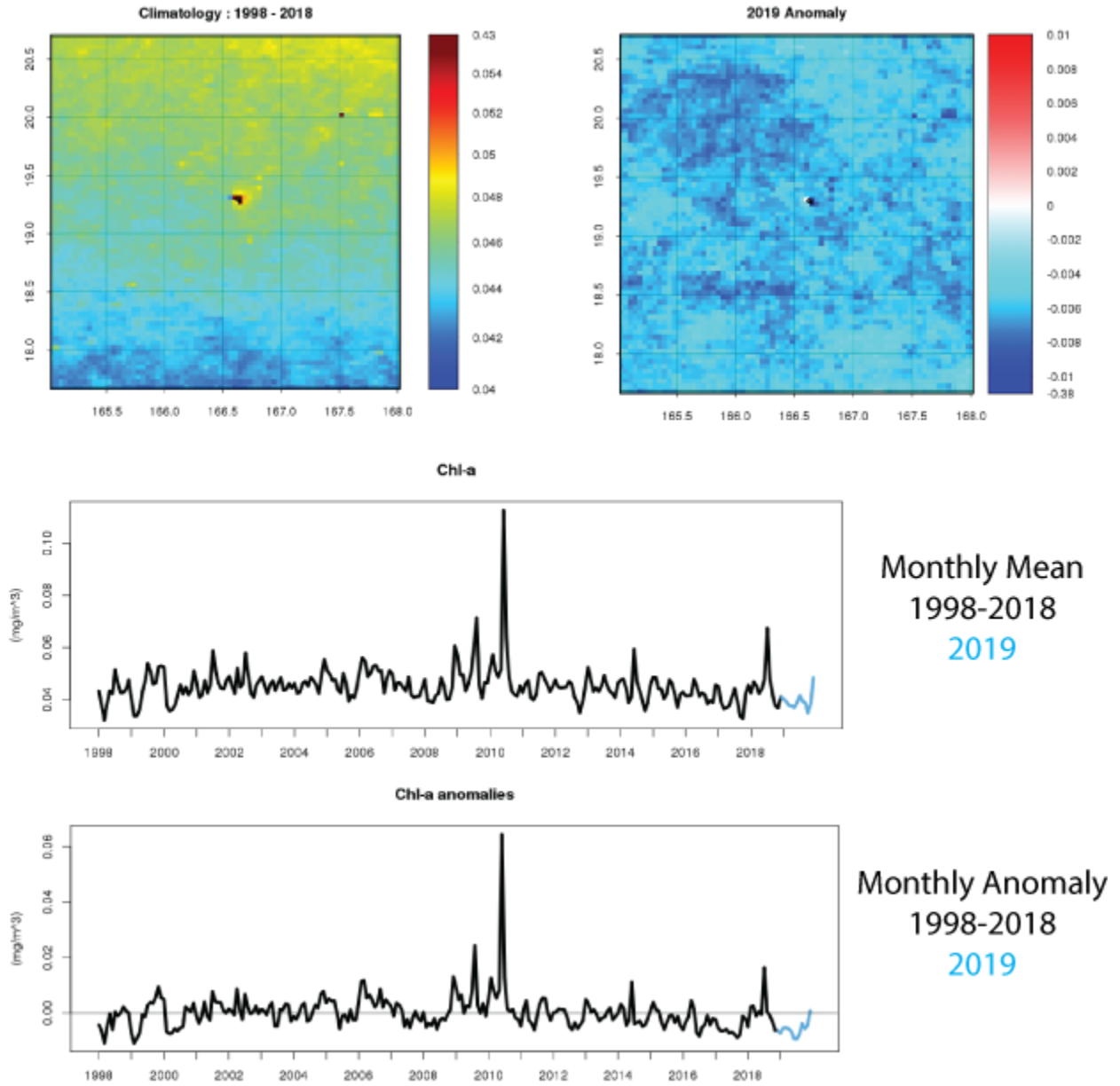
Figure 20. Chlorophyll-A (Chl-A) and Chl-A Anomaly from the Wake Atoll Grid
