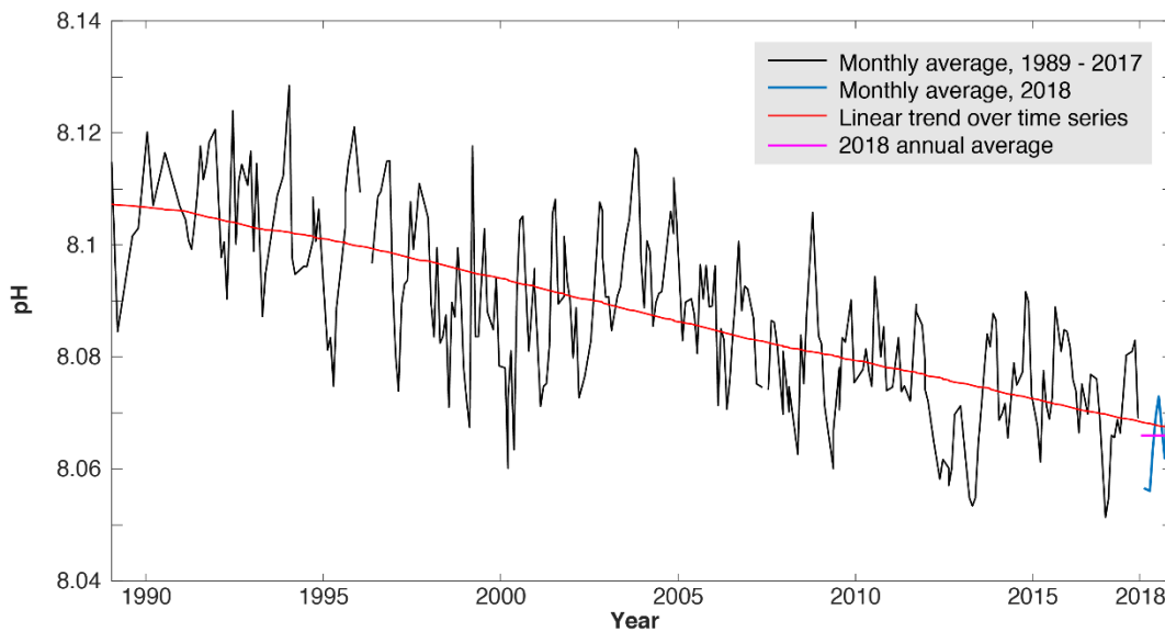
Figure 6. Oceanic pH (black) and its trend (red) at Station ALOHA from 1989 – 2018
