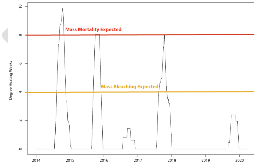
Figure 17. Coral Thermal Stress Exposure, Wake Atoll Virtual Station 2013-2018 (Coral Reef Watch Degree Heating Weeks)
