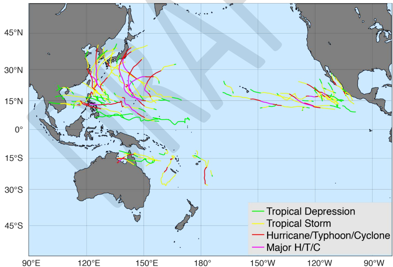
Figure 9. 2019 Pacific basin tropical cyclone tracks
