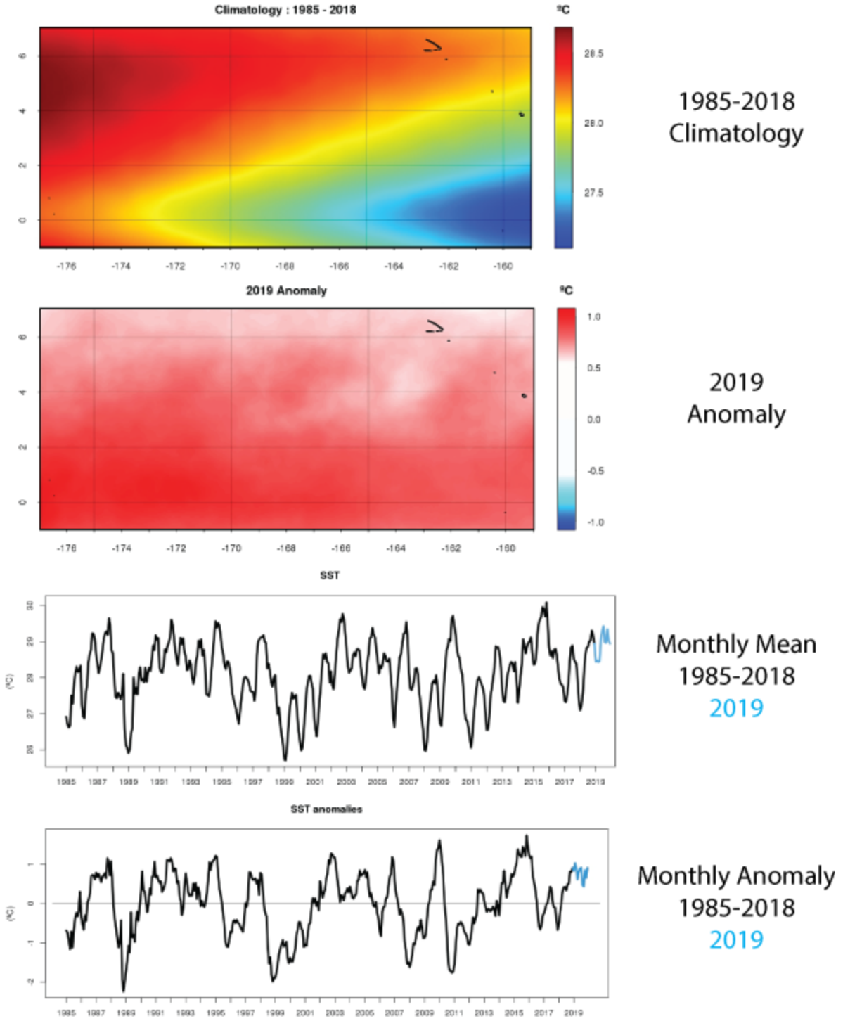
Figure 11. Sea surface temperature climatology and anomalies from the PRIA Grid
