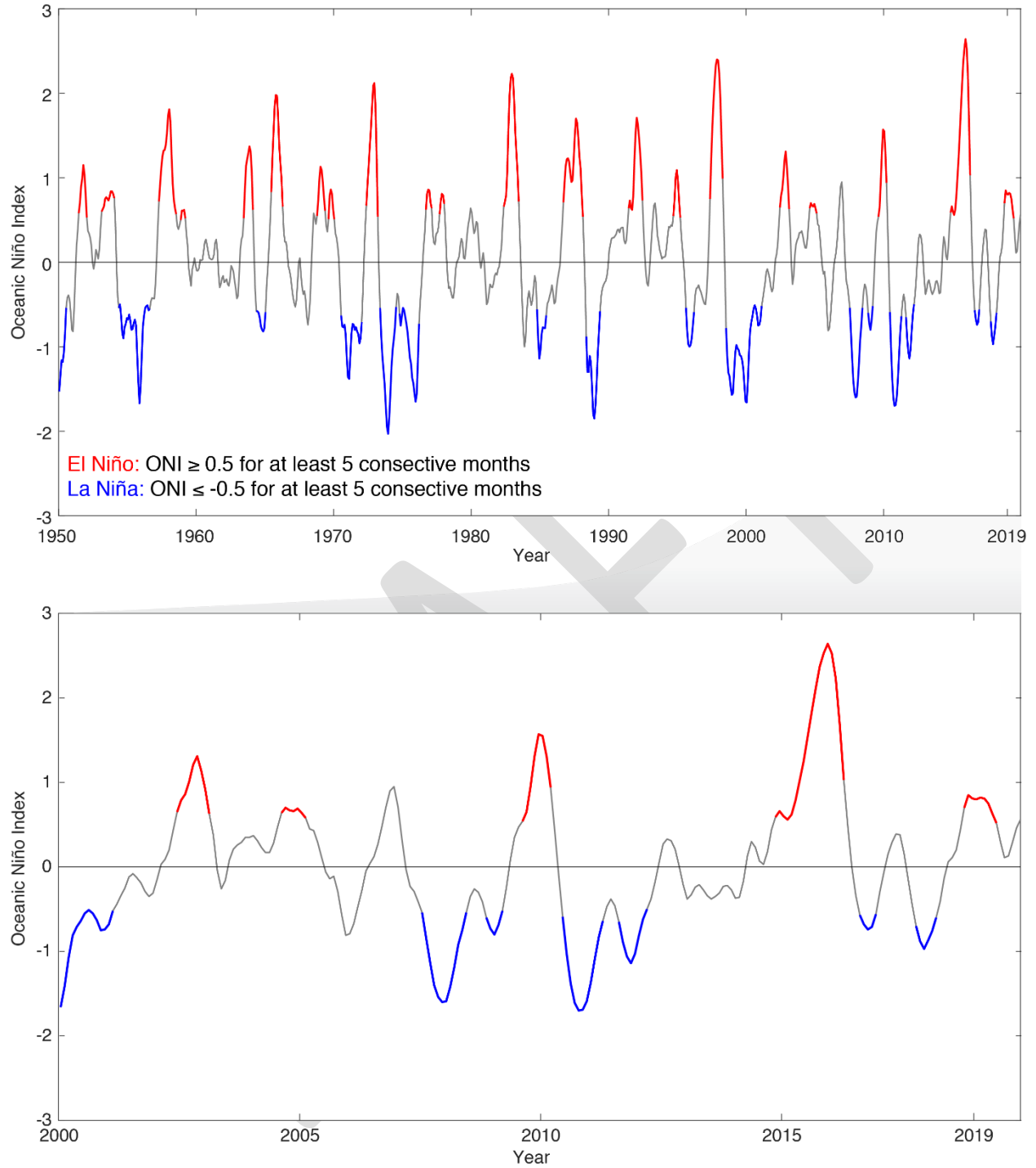
Figure 7. Oceanic Niño Index from 1950-2019 (top) and 2000–2019 (bottom) with El Niño periods in red and La Niña periods in blue
