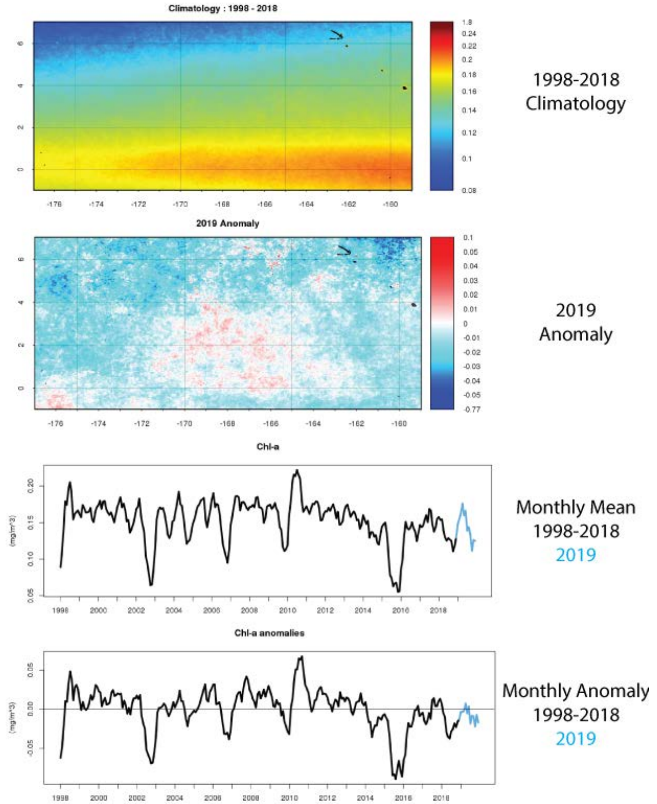
Figure 18. Chlorophyll-A (Chl-A) and Chl-A Anomaly from the PRIA Grid
