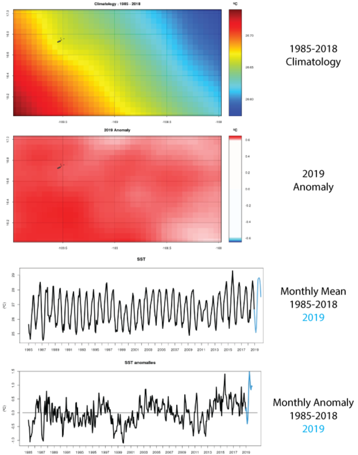
Figure 12. Sea surface temperature climatology and anomalies from Johnston Atoll Grid
