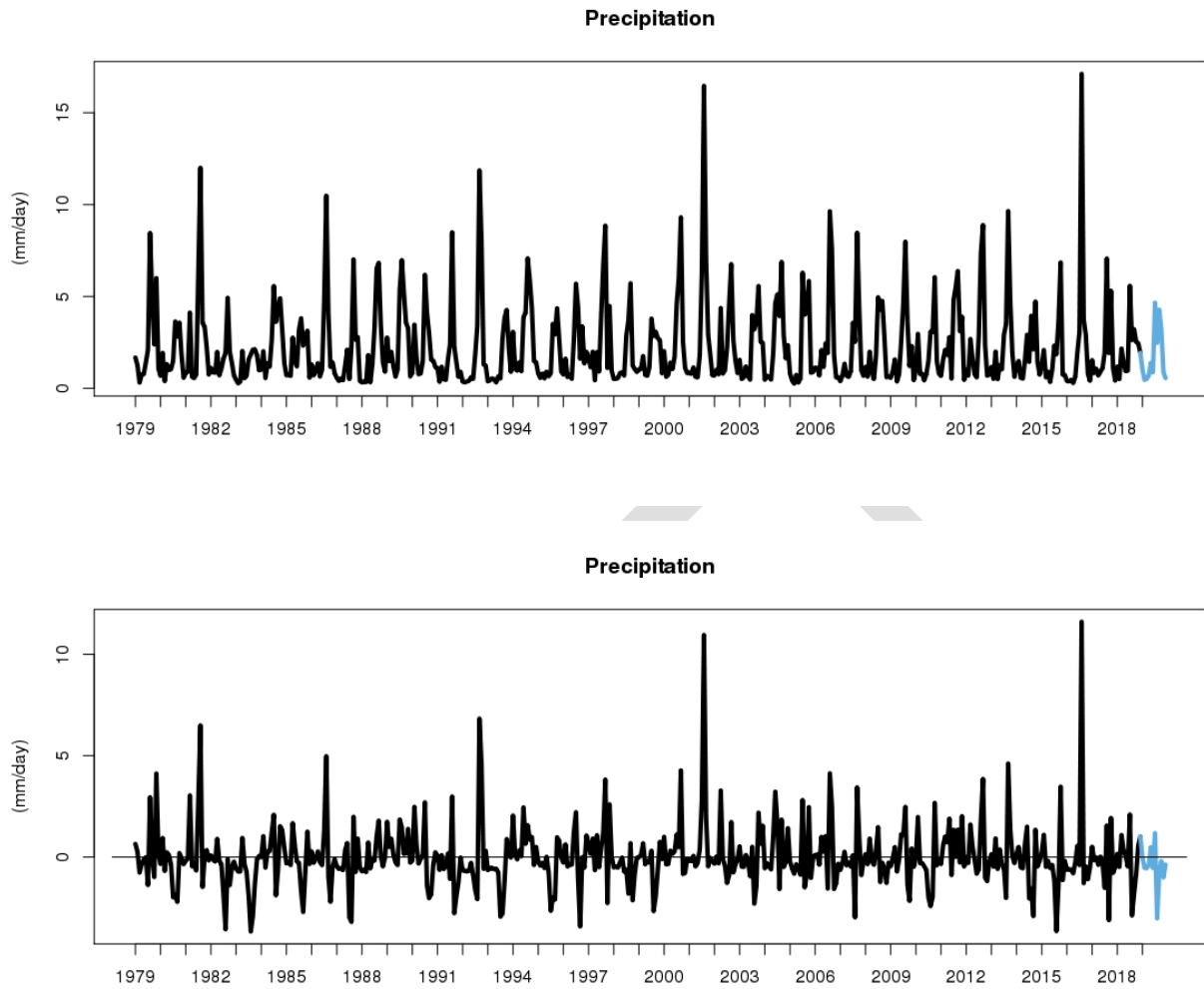
Figure 23. CMAP precipitation across the Wake Atoll Grid with 2019 values in blue
