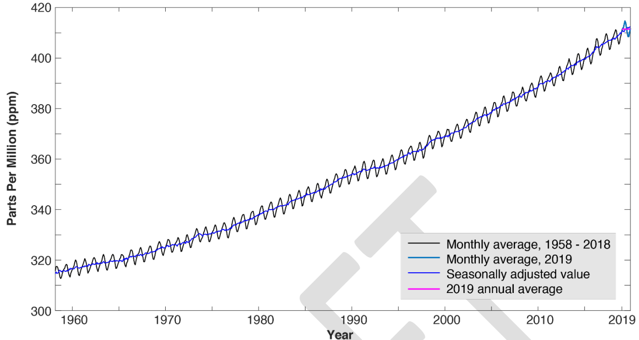
Figure 5. Monthly mean (black) and seasonally corrected (blue) atmospheric carbon dioxide at Mauna Loa Observatory, Hawaii
