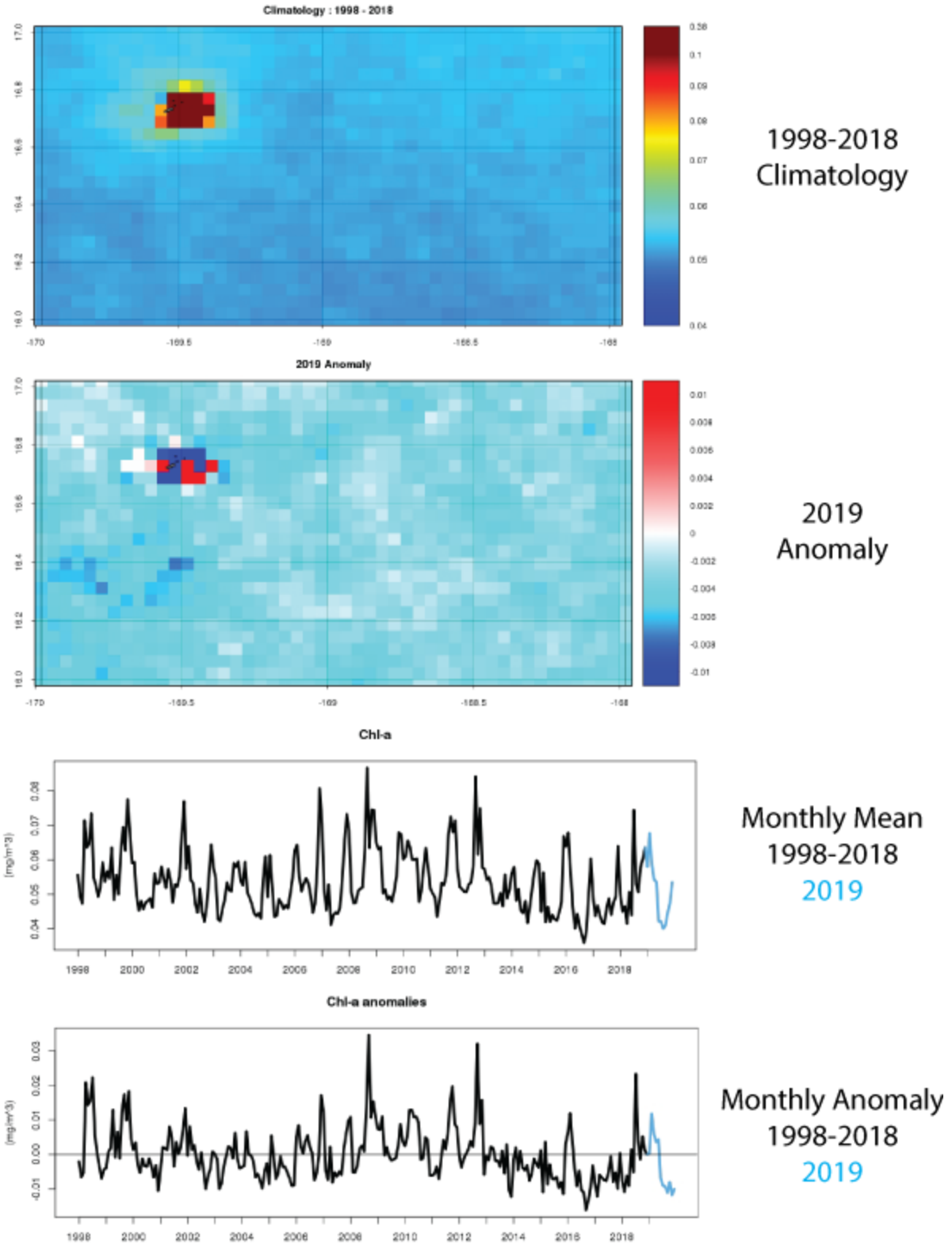
Figure 19. Chlorophyll-A (Chl-A) and Chl-A Anomaly from the Johnston Atoll Grid
