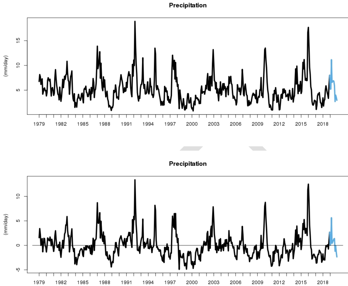
Figure 21. CMAP precipitation across the PRIA Grid with 2019 values in blue
