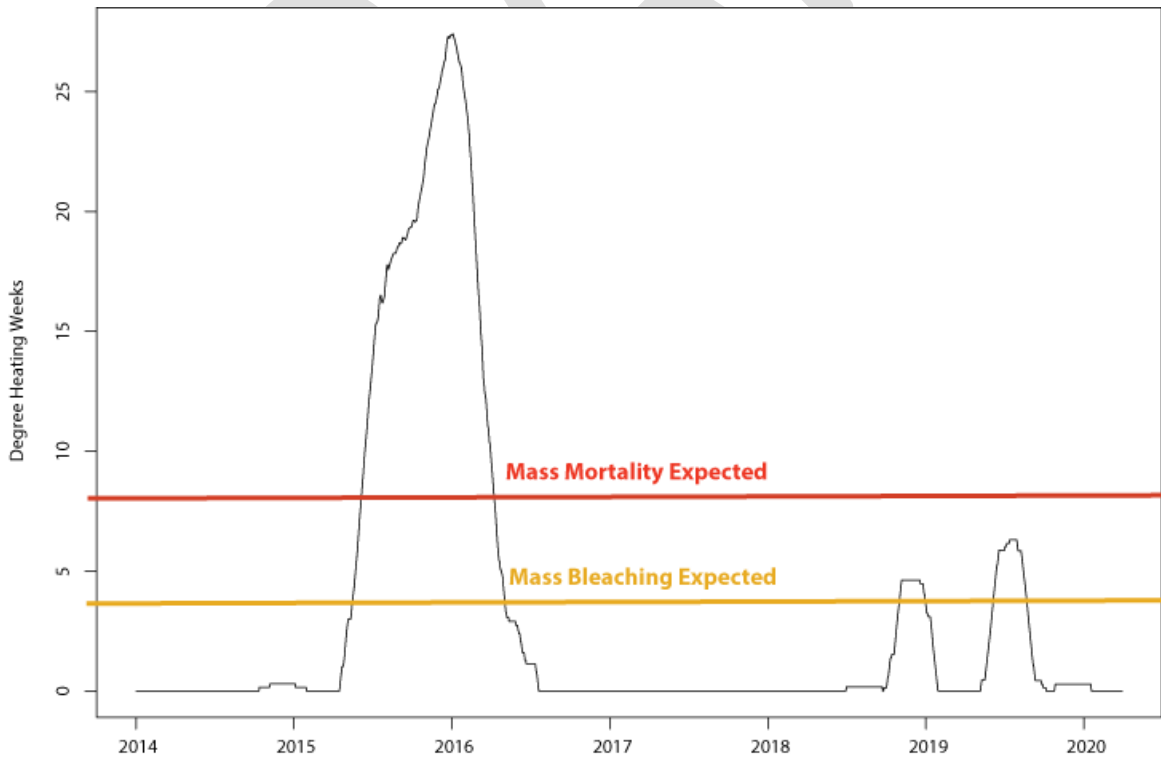
Figure 15. Coral Thermal Stress Exposure, Northern Line Islands Virtual Station 2014-2019 (Coral Reef Watch Degree Heating Weeks)
