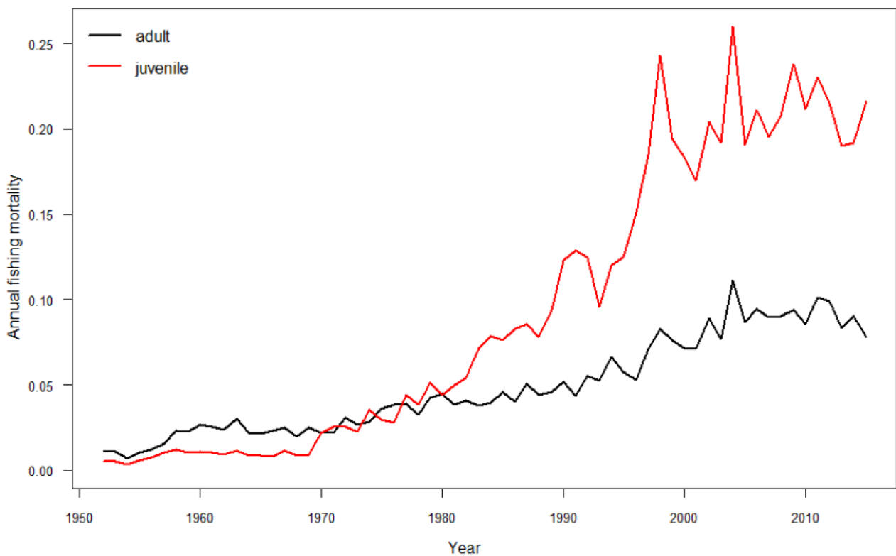
Figure 12: Estimated annual average juvenile and adult fishing mortality for the diagnostic case model (WCPFC 2018).
