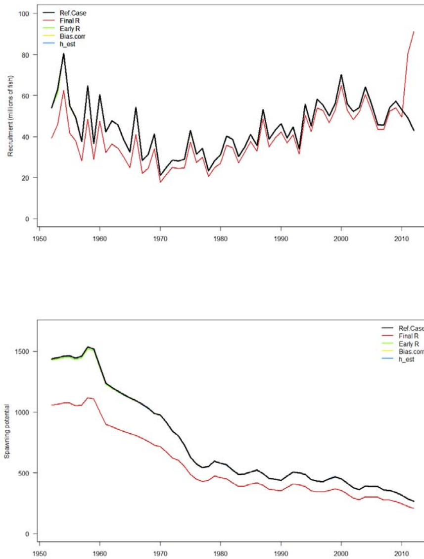
Figure 10.4 1: Estimated annual recruitment (top) and spawning potential (bottom) for the WCPO obtained from runs described in Table 10.4 1.
