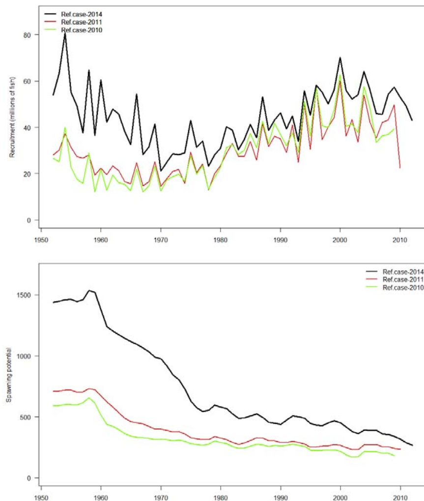
Figure 10.2 2: Annual recruitment (top) and spawning biomass (bottom) estimates from the reference case models used for the WCPO bigeye assessments from 2010, 2011 and the current assessment (2014).
