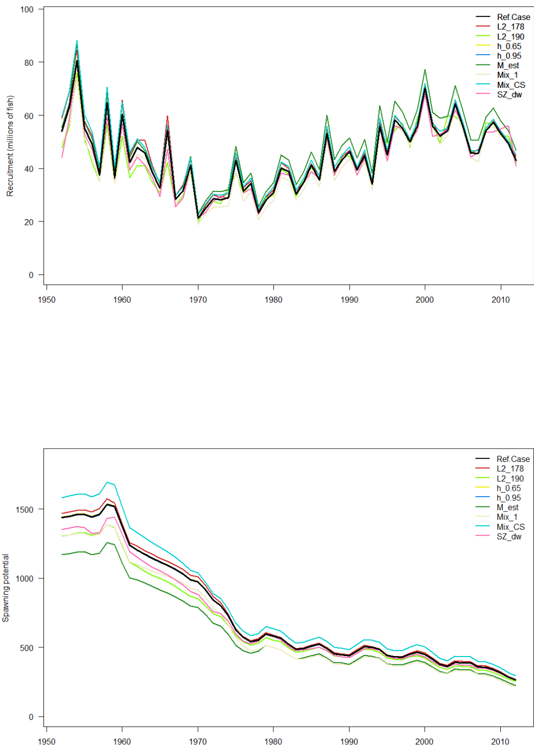
Figure 39. Estimated average recruitment (top) and spawning potential (bottom) for the WCPO obtained from the one-off sensitivity model runs to the reference case (see Table 5 for details of each scenario).
