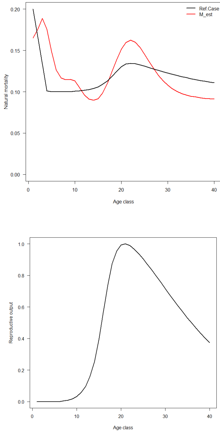
Figure 9. Natural mortality-at-age as assumed in the reference case and estimated in the one-change sensitivity (top) and % mature (bottom) . Note that the estimate of maturity is actually used to define an index of spawning potential incorporating information on sex ratios, maturity at age, fecundity, and spawning fraction (see Hoyle and Nicol 2008 for further details).
