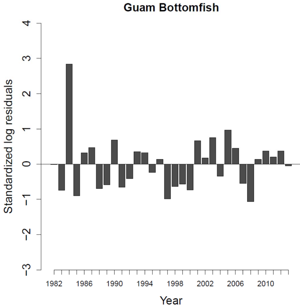
Figure 12. Residuals of production model fit to nominal observed CPUE for Guam bottomfish, 1982-2013.
