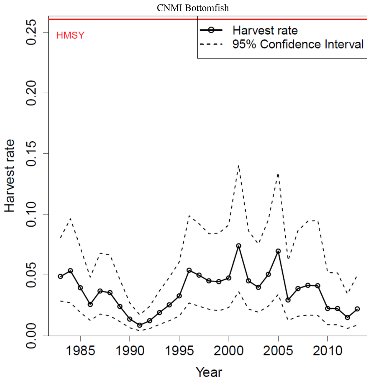
Figure 17. CNMI bottomfish harvest rates: Model-estimated trends in mean annual harvest rate (black circles, solid line) with 95% confidence intervals (black dotted line). The overfishing limit of HMSY is indicated with a horizontal solid red line. Harvest rate estimates were generally below the overfishing limit, indicating overfishing was not and is not occurring.
