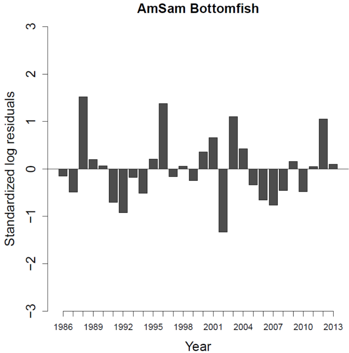
Figure 8. Residuals of production model fit to nominal observed CPUE for American Samoa bottomfish, 1986-2013.
