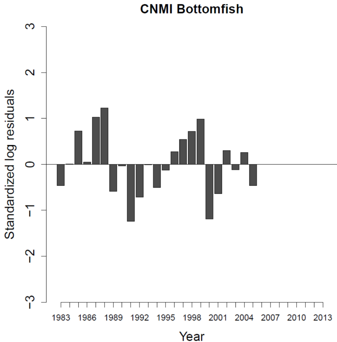
Figure 10. Residuals of production model fit to nominal observed CPUE for CNMI bottomfish, 1983-2005.
