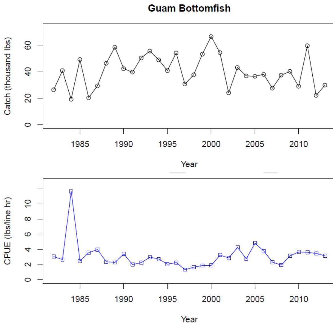
Figure 6. (top) Final catch (thousand lbs) of Guam BMUS (Bottomfish Management Unit Species Complex) from 1982-2013 used in this stock assessment update. (bottom) Final nominal catch per unit effort (CPUE, in lbs/line hour) of Guam BMUS (Bottomfish Management Unit Species Complex) from 1982-2013 used in this stock assessment update.
