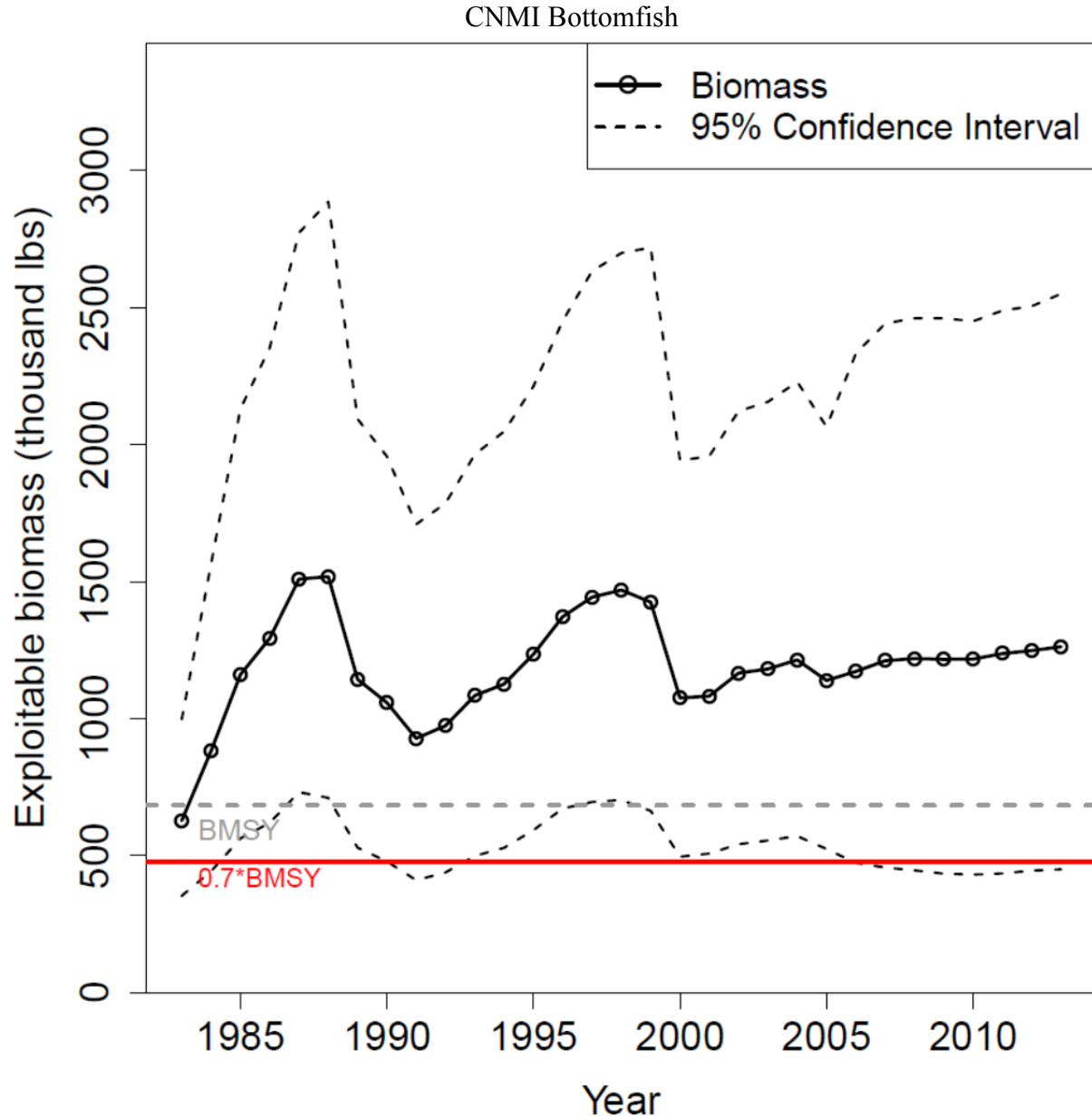
Figure 16. CNMI bottomfish biomass: Model-estimated trends in mean values (black circles, solid line) with 95% confidence intervals (black dotted line). BMSY is indicated with a horizontal gray dotted line, and the overfished limit of 0.7 \times \text{BMSY} is indicated with a horizontal solid red line. Biomass estimates were generally above the overfished limit with the exception of a few years. In recent years the stock status is not considered to be overfished.
