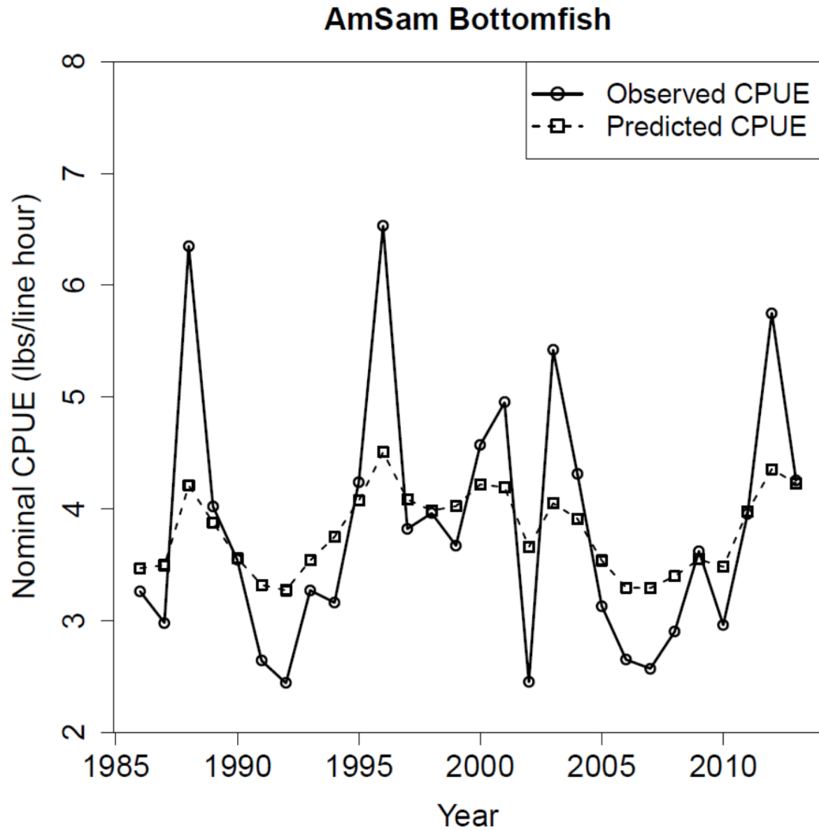
Figure 7. Comparison of observed nominal CPUE (circles with solid line) with model-predicted nominal CPUE (squares with dotted line) of American Samoa bottomfish, 1986-2013.
