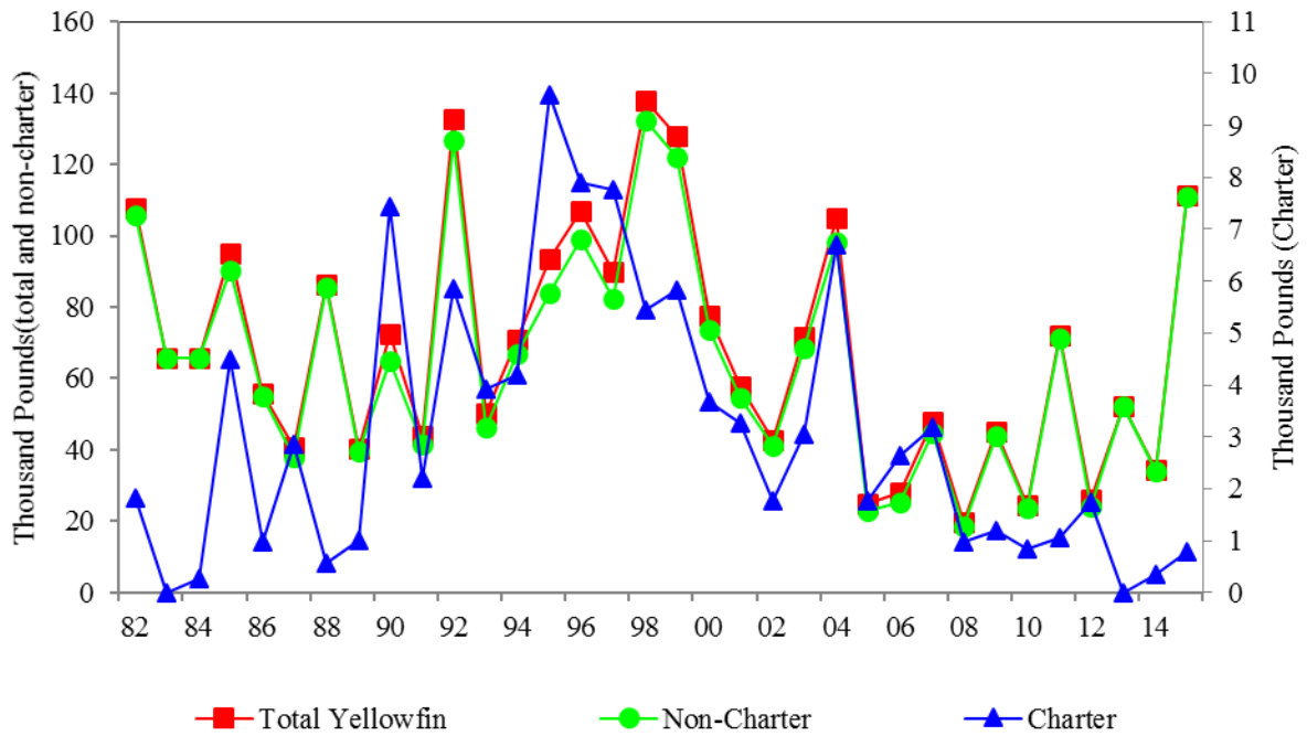
Figure 56. Guam Annual Estimated Total Yellowfin Landings by Method
