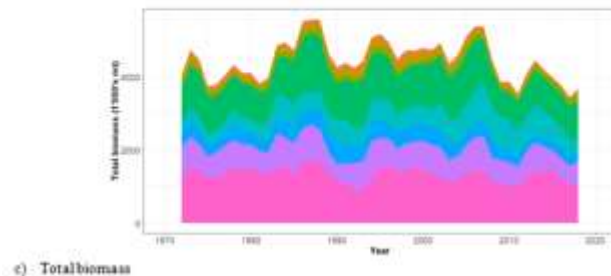
Figure SKJ-04. Estimated annual average recruitment, spawning potential and total biomass by model region for the diagnostic model, showing the relative sizes among regions.
