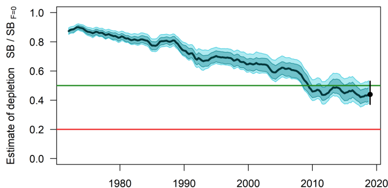
Figure SKJ-08. Plot showing the trajectories of spawning potential depletion for the model runs included in the structural uncertainty grid weighted by the values given in Table SKJ-01. Red horizontal line indicates the agreed limit reference point, the green horizontal line indicates the interim target reference point.
