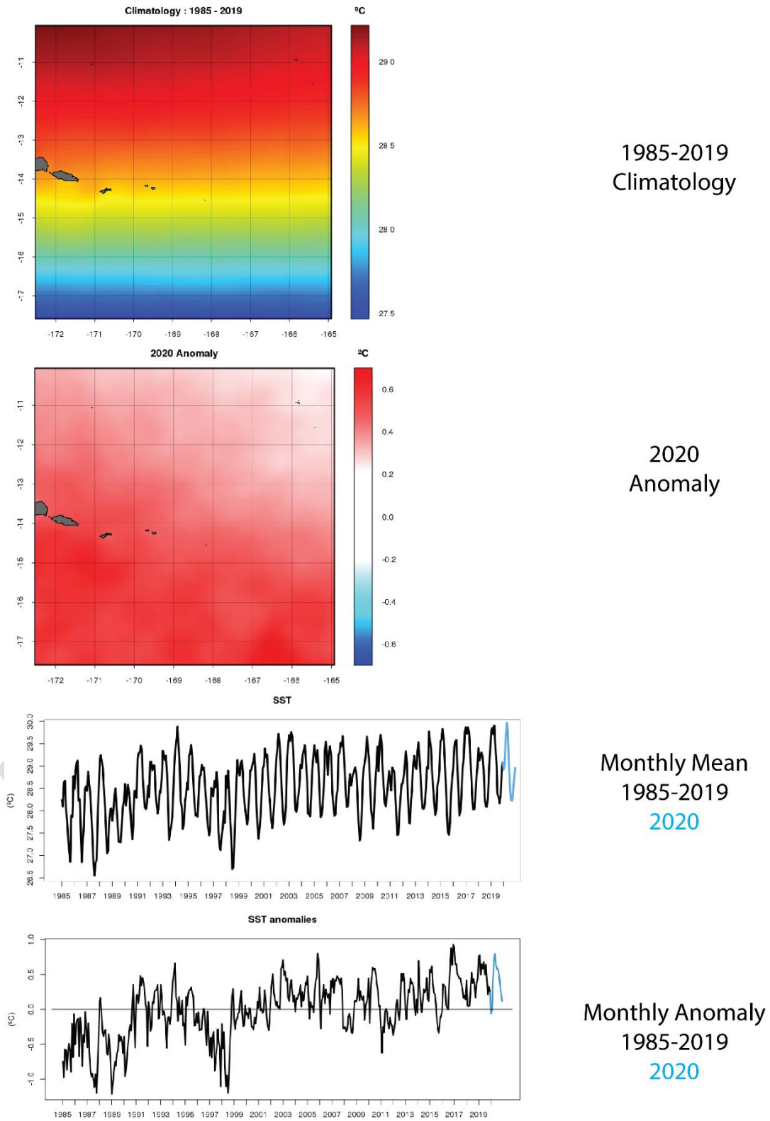
Figure 11. Sea surface temperature climatology and anomalies from 1985-2020
