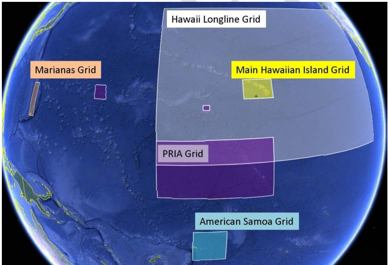
Figure 4. Regional spatial grids representing the scale of the climate change indicators being monitored
