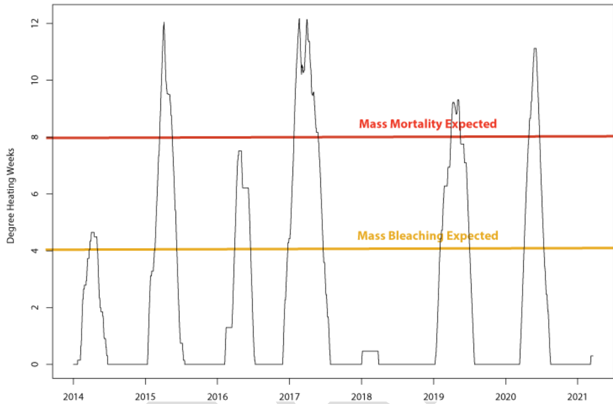
Figure 12. Coral Thermal Stress Exposure measured at Samoa Virtual Station 2014-2020 (Coral Reef Watch Degree Heating Weeks)
