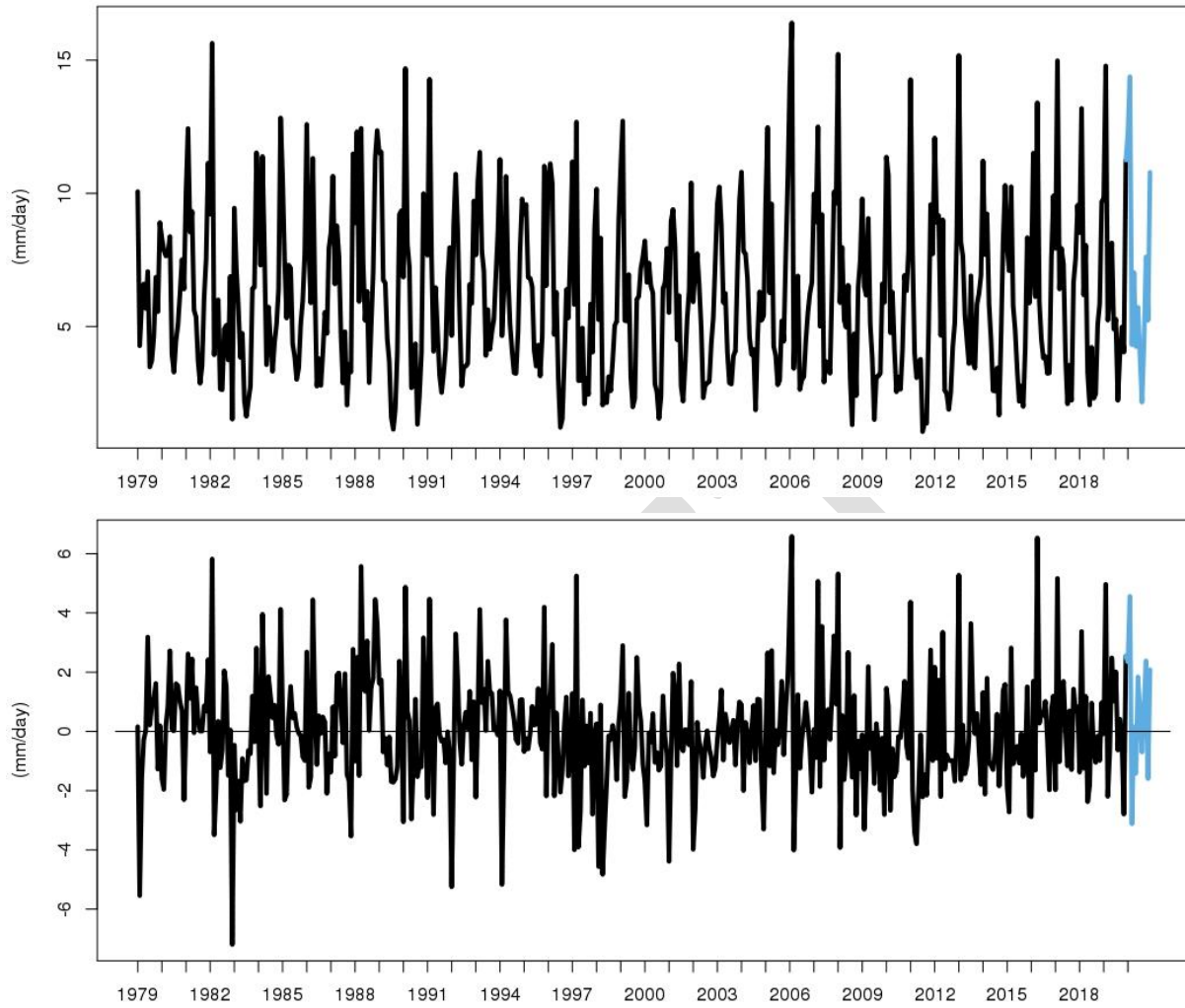
Figure 14. CMAP precipitation (top) and anomaly (bottom) across the American Samoa Longline Grid with 2020 values in blue
