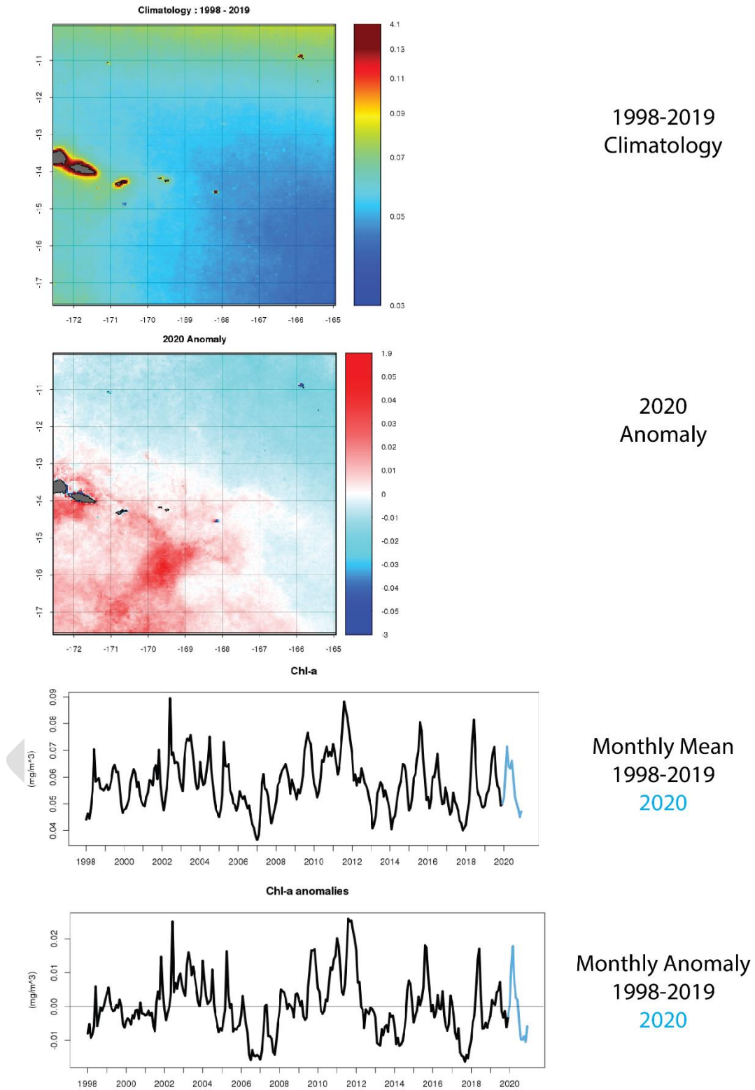
Figure 13. Chlorophyll-a and Chlorophyll-a Anomaly from 1998-2020
