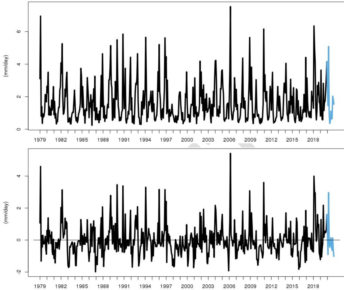
Figure 14. CMAP precipitation (top) and anomaly (bottom) across the MHI Grid with 2020 values in blue
