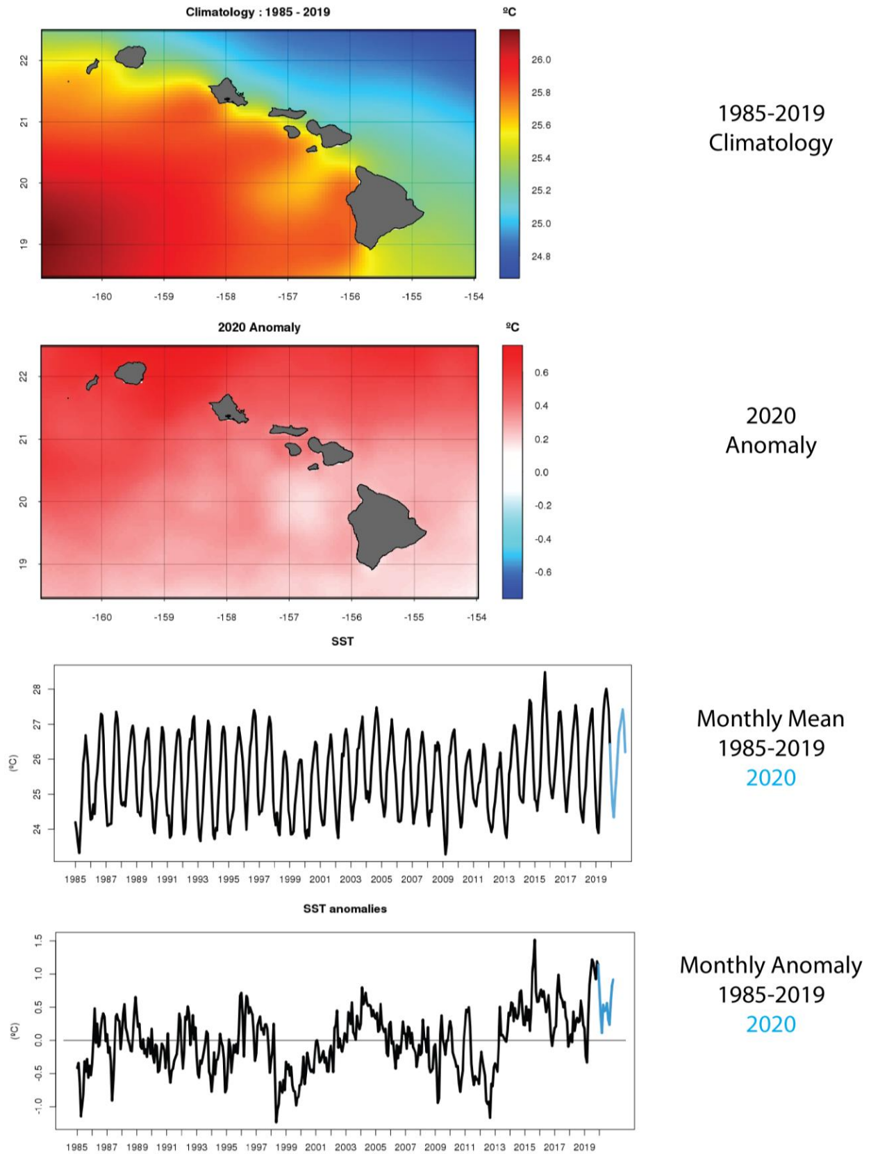
Figure 11. Sea surface temperature climatology and anomalies from 1985-2020
