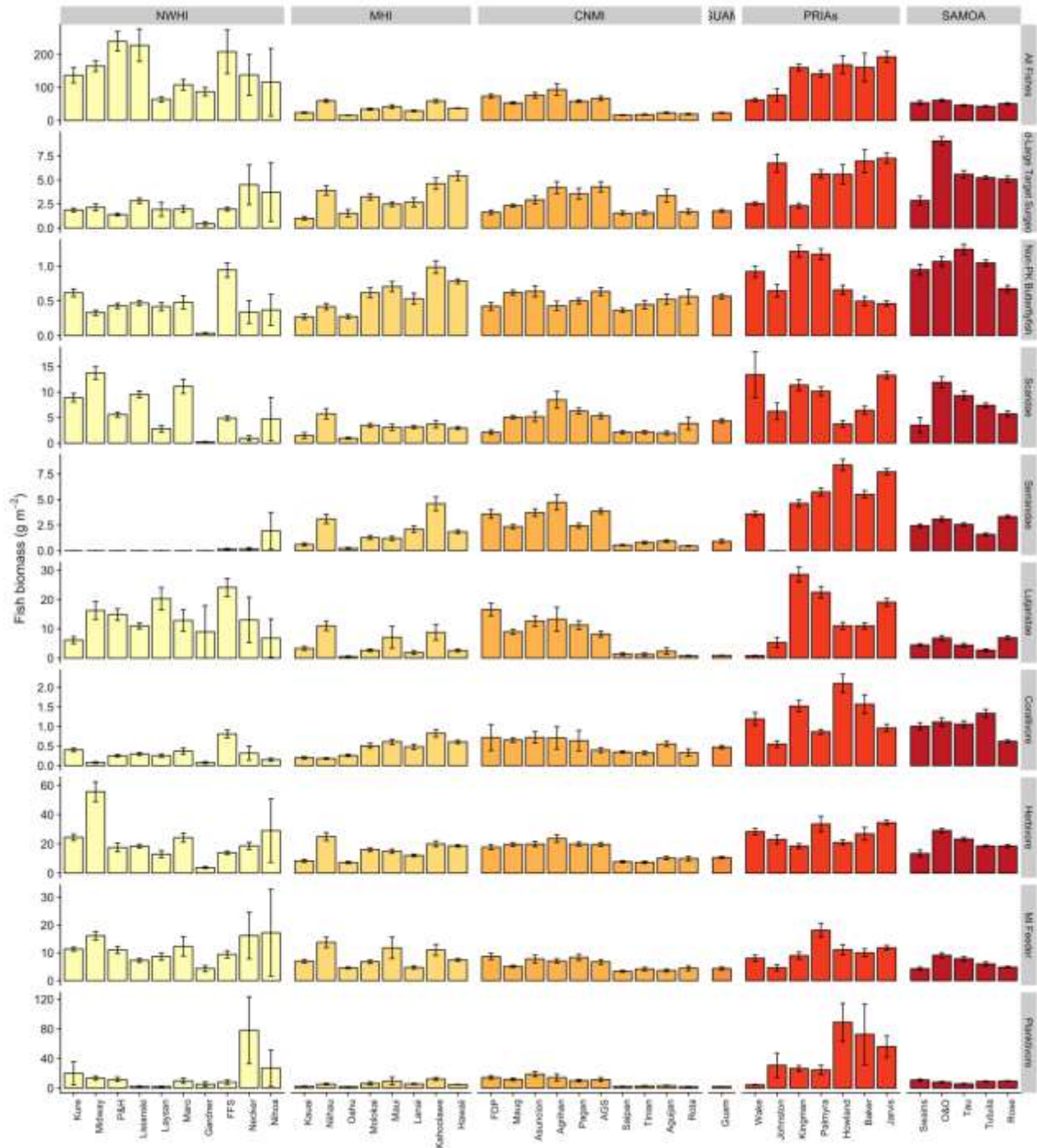
Figure 7. Mean fish biomass ( \text{g m}^{-2} \pm \text{standard error} ) of functional, taxonomic, and trophic groups by U.S. Pacific reef area from the years 2010-2020 by latitude. The group Serranidae excludes planktivorous members of that family – i.e., anthias, which can be hyper-abundant in some regions. Similarly, the bumphead parrotfish, Bolbometopon muricatum , has been excluded from the corallivore group – as high biomass of that species at Wake overwhelms corallivore biomass at all other locations. The group “MI Feeder” consists of fishes that primarily feed on mobile invertebrates
