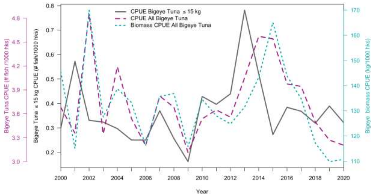
Figure 182. Annual CPUE of bigeye tuna \leq 15 kg (grey solid line), CPUE of all bigeye tuna (pink dashed line), and biomass CPUE (blue dotted line) from 2000 – 2020, all from deep sets
