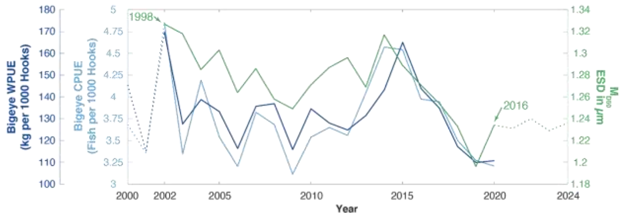
Figure 183. Annual WPUE (dark blue) and CPUE (light blue) of bigeye tuna from deep sets, as well as four-year lagged median phytoplankton size ( M_{D50} , green). Dashed lines indicate years that are outside the forecast period described in the text
