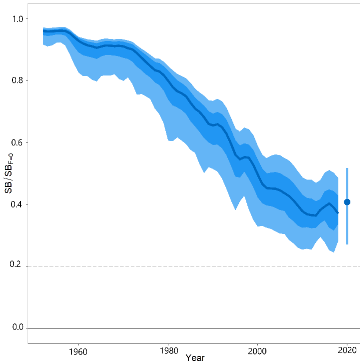
Figure BET-8. Time-dynamic percentiles of depletion ( SB_t/SB_{F=0} ) and median (dark line) across all 24 models in the structural uncertainty grid. The lighter band shows the 10 th to 90 th percentiles around the median, and the dark band shows the 50 th percentile around the median. The median SB_{recent}/SB_{F=0} and 80 th percentile is shown on the right by the dot and line.
