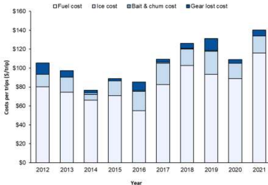
Figure 131. Average trip costs for American Samoa trolling trips from 2012–2021 adjusted to 2021 dollars 1
