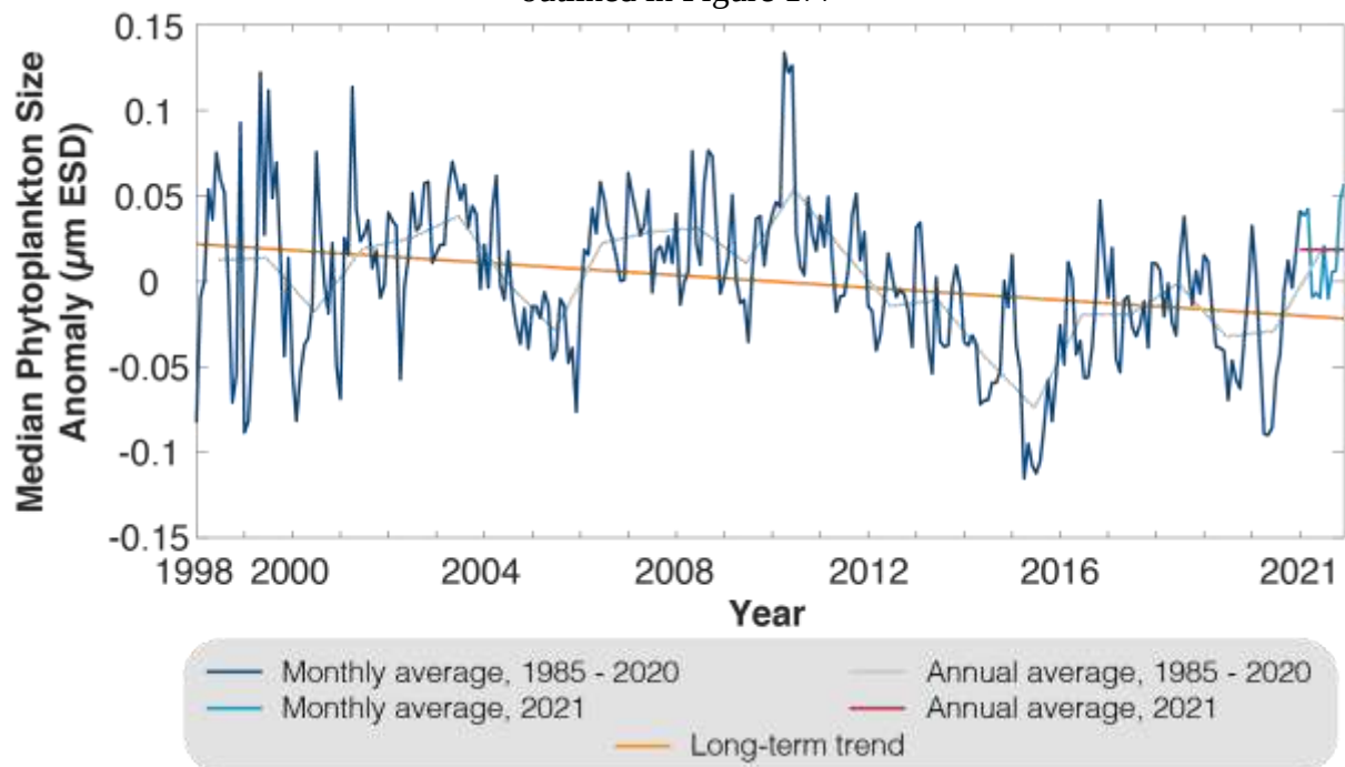
Figure 177. Time series of monthly median phytoplankton size anomaly over the longline fishing grounds outlined in Figure 176
