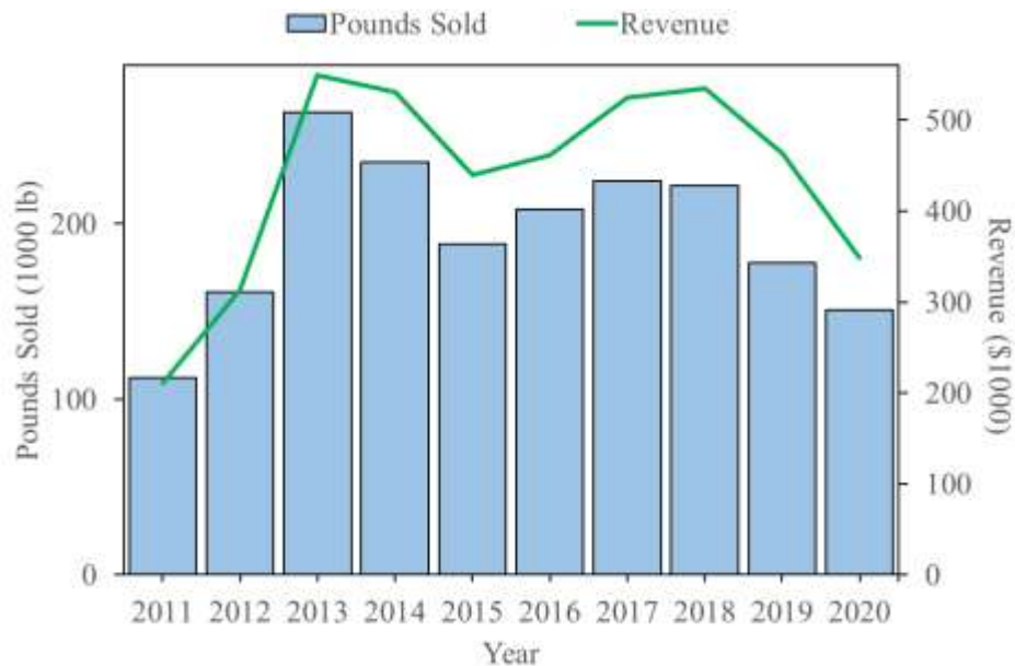
Figure 132. Total PMUS annual pounds sold and revenues in the CNMI for all gears from 2011-2020 adjusted to 2020 dollars 1
