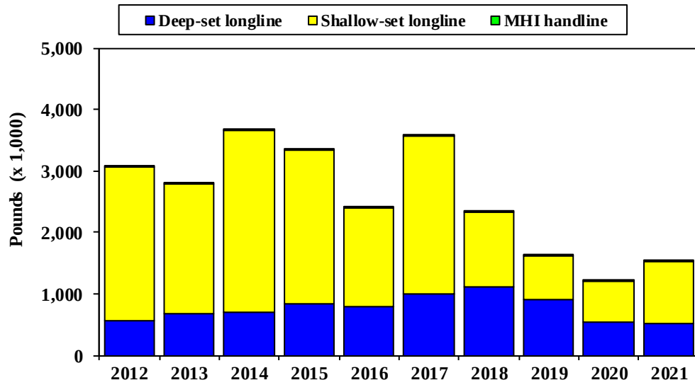
Figure 77. Hawaii swordfish catch by gear type Supporting data shown in Table A-78.
