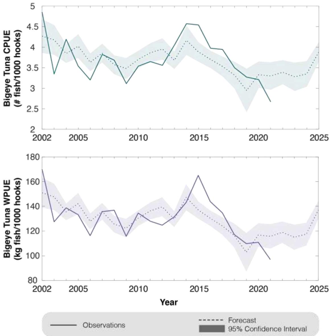
Figure 183. Annual observed (solid lines) and forecast (dotted lines) CPUE (upper panel; green) and WPUE (lower panel; purple) of bigeye tuna from deep sets. The forecasts' 95% confidence intervals are shaded
