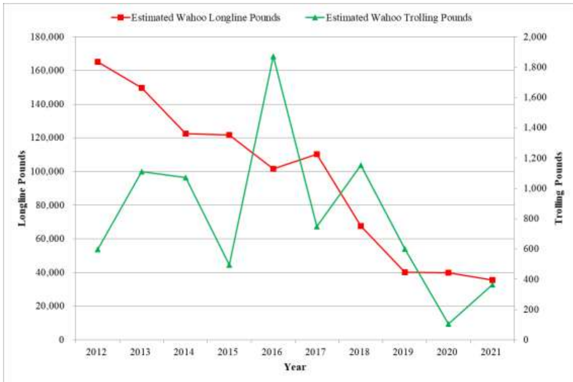
Figure 8. Total estimated landings of wahoo in American Samoa Unrepresentative amount of wahoo catch from trolling one day in 2016. Supporting data shown in Table A-8.
