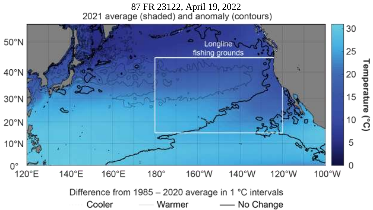
Figure 167. Average 2021 sea surface temperature (shaded) and the difference from the 1985 – 2020 average (contoured). The white rectangle identifies the area targeted by Hawaii’s longline fisheries. SST is averaged over this area for the time series shown in Figure 168 and Figure 169
