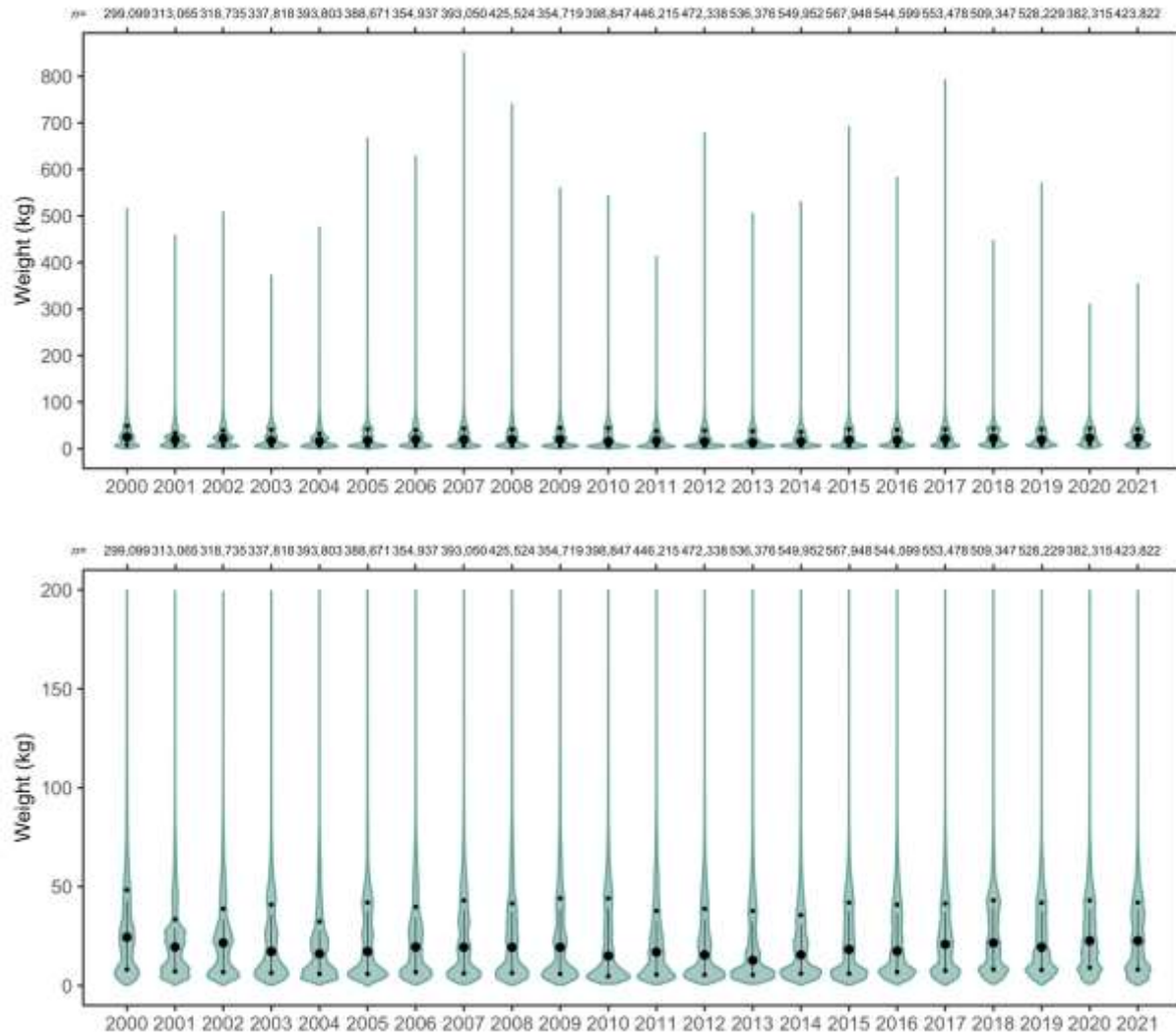
Figure 179. The annual distribution of weights of all fish, showing the full range of weights (top) and truncated to better demonstrate the distribution of the majority of weights (bottom) with large circles denoting median weight, black lines showing the range of the middle 50% of fish, small circles denoting the 20 th and 80 th percentiles of the weight distributions, and width of shading proportional to the number of fish of a given weight
