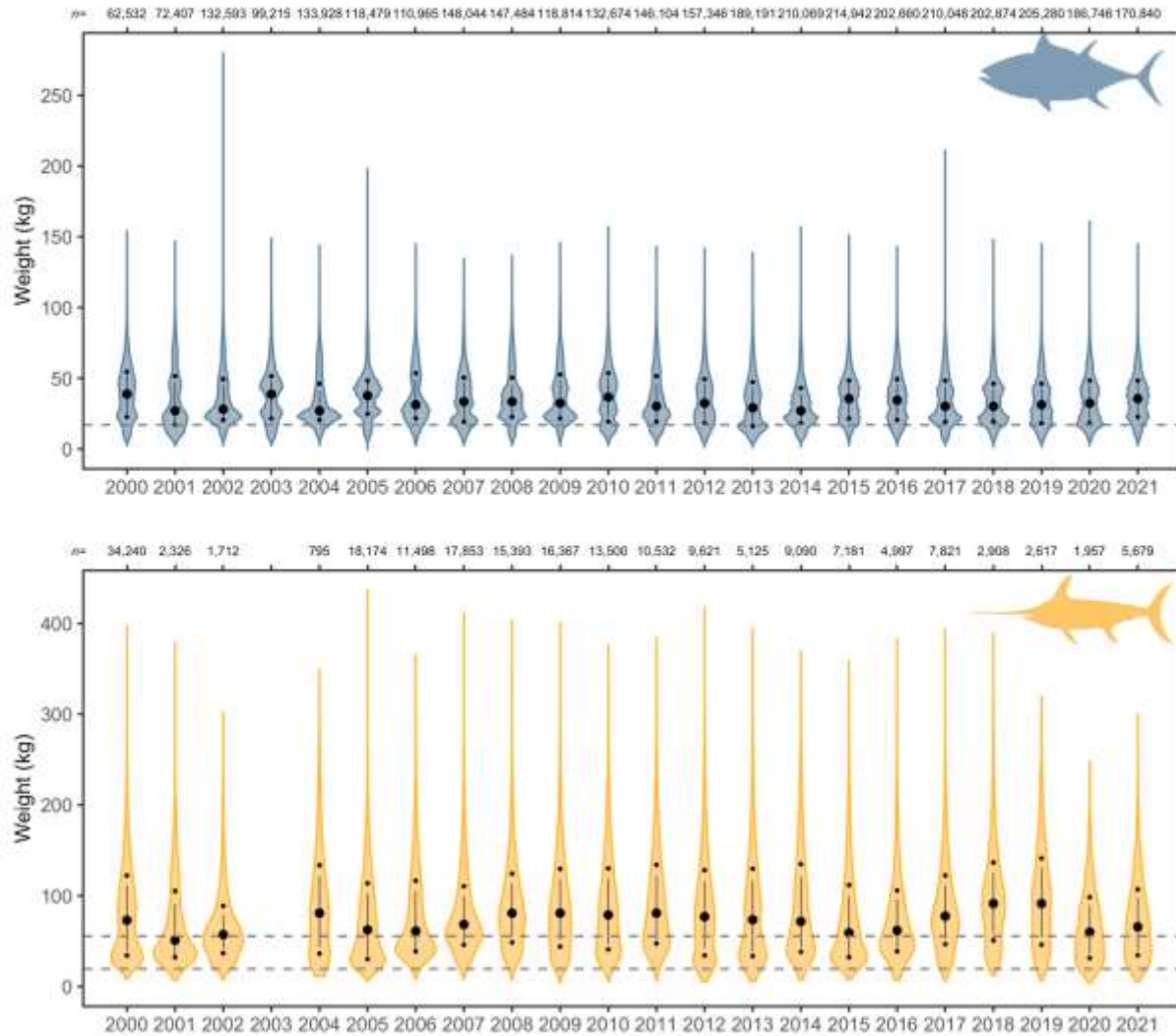
Figure 180. The annual distribution of weights of bigeye tuna from deep sets (top) and swordfish from shallow sets (bottom), with large circles denoting median weight, black lines showing the range of the middle 50% of fish, small circles denoting the 20 th and 80 th percentiles of the weight distributions, and width of shading proportional to the number of fish of a given weight. Horizontal dashed lines denote the weight corresponding to L_{50} for bigeye tuna (17 kg; Farley et al. 2018), female swordfish (55.5 kg; Kapur et al. 2017), and male swordfish (19.4 kg, Kapur et al. 2017)
