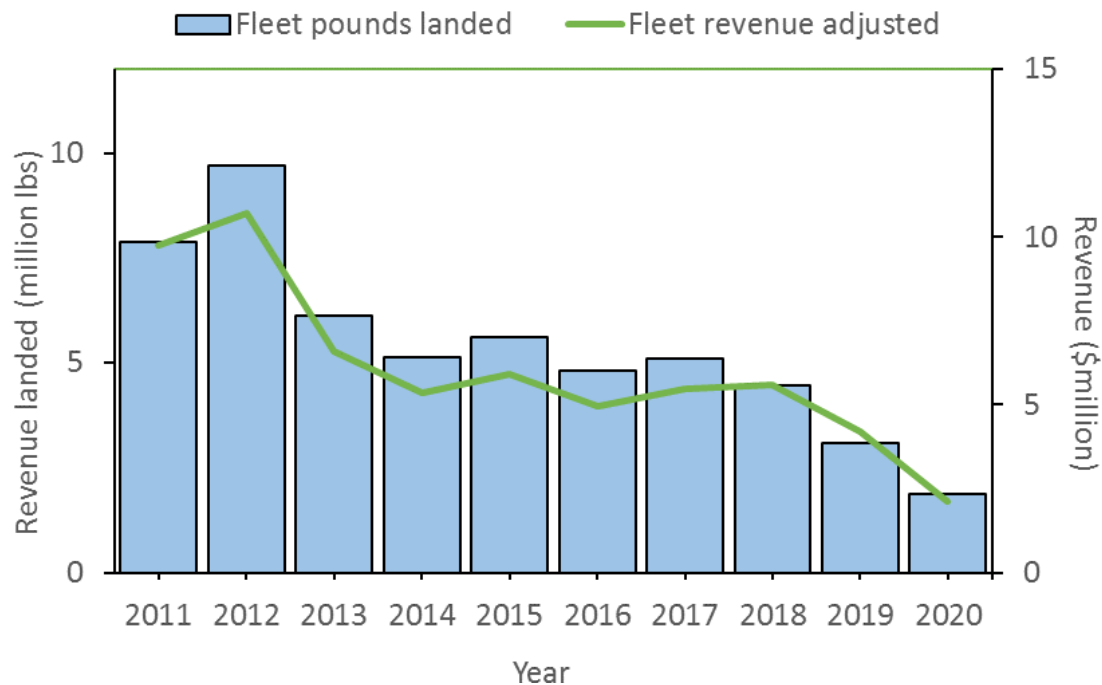
Figure 122. Commercial landings and revenues of the American Samoa longline fishery from 2011-2020 adjusted to 2020 dollars 1
