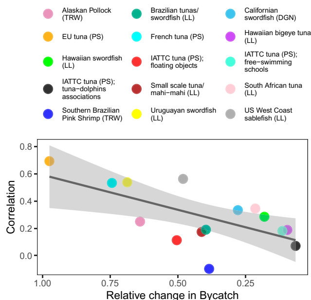
Fig. 7. Relationship between predicted bycatch reduction (x-axis) and correlation between total bycatch and total target species (y-axis). Bycatch reduction indicates relative change compared to no closure ( = 1 ). Each dot represents a different case study, and this plot shows, as an example, the results from a 30% closed area in a dynamic mosaic approach. The solid line represents a simple regression and the gray area the 95% CI. LL: Long-line; DGN: Drift Gillnet; TRW: Trawling; PS: Purse-seine. US: United States; EU: European Union; IATTC: Inter-American Tropical Tuna Commission.
