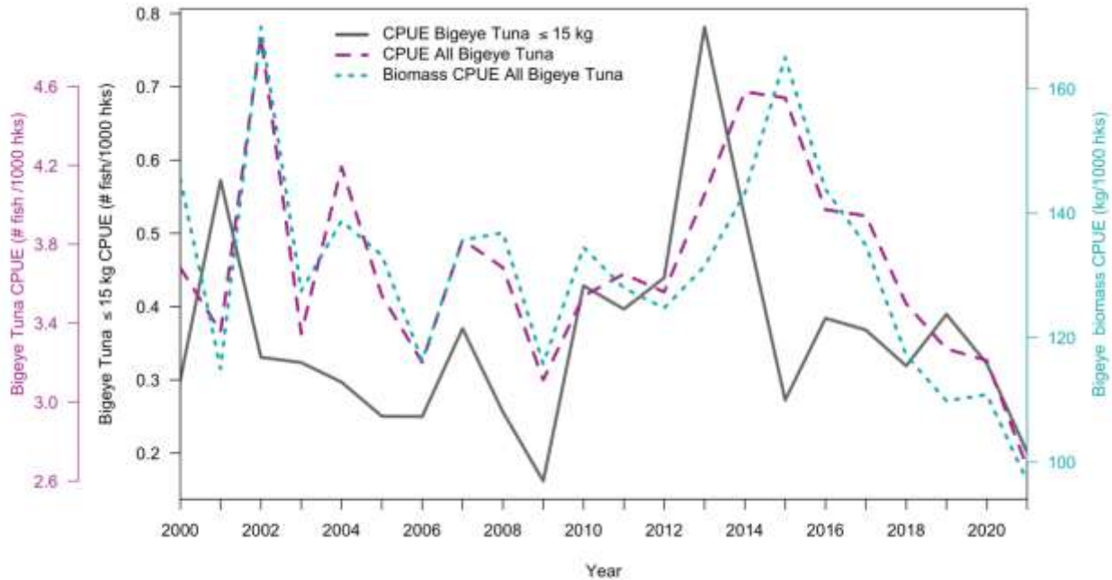
Figure 182. Annual CPUE of bigeye tuna ≤ 15 kg (grey solid line), CPUE of all bigeye tuna (pink dashed line), and biomass CPUE (blue dotted line) from 2000 – 2021, all from deep sets
