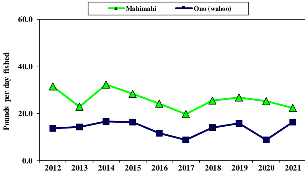
Figure 103. Mahimahi and Ono CPUE for the MHI troll fishery
