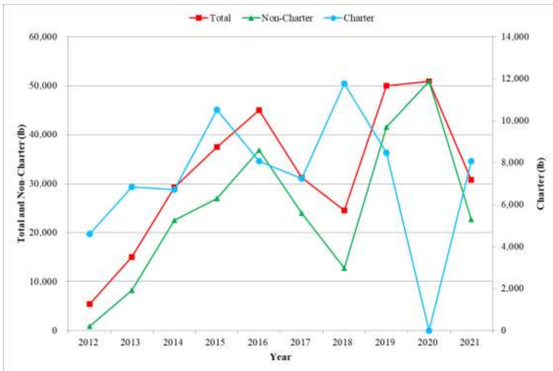
Figure 56. Total estimated landings for blue marlin in Guam
