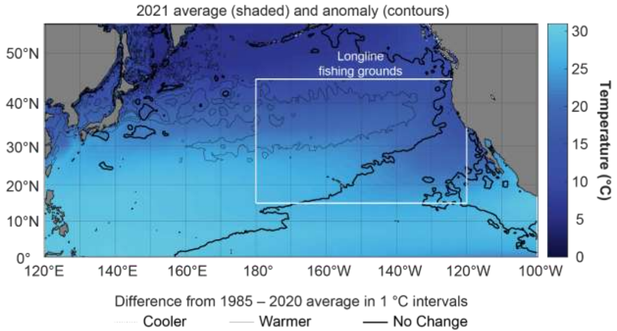
Figure 167. Average 2021 sea surface temperature (shaded) and the difference from the 1985 – 2020 average (contoured). The white rectangle identifies the area targeted by Hawaii’s longline fisheries. SST is averaged over this area for the time series shown in Figure 168 and Figure 169
