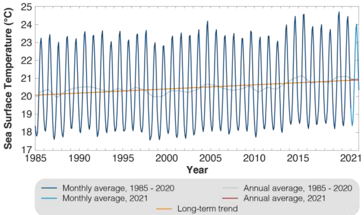
Figure 168. Time series of monthly average sea surface temperature over the longline fishing grounds outlined in Figure 167
