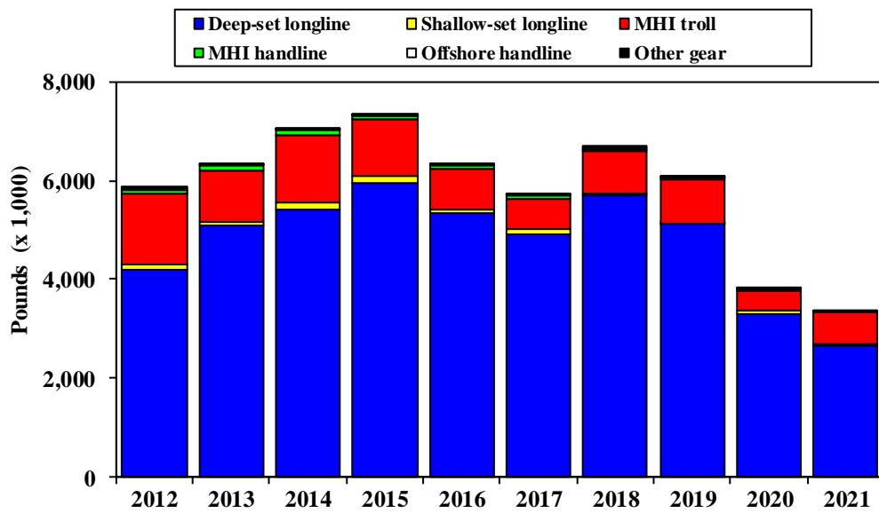
Figure 80. Hawaii commercial catch of other PMUS by gear type
