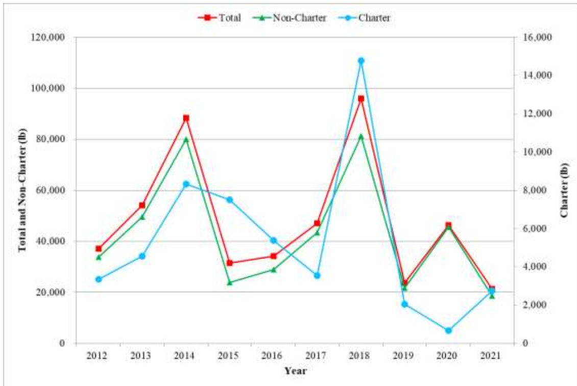
Figure 55. Total estimated landings for wahoo in Guam
