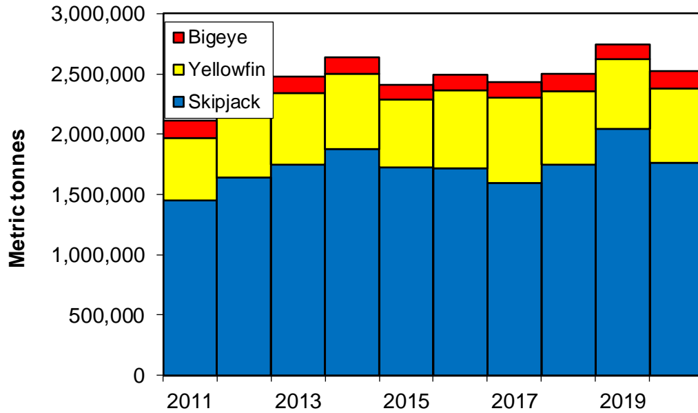
Figure 115. Total purse seine catch of skipjack, yellowfin, and bigeye tuna in the Pacific Ocean
