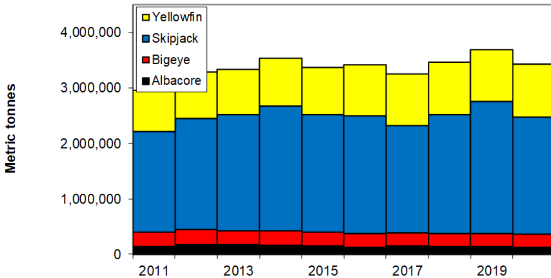
Figure 114. Estimated total annual catch of tuna species in the Pacific Ocean Source: SPC (2021).
