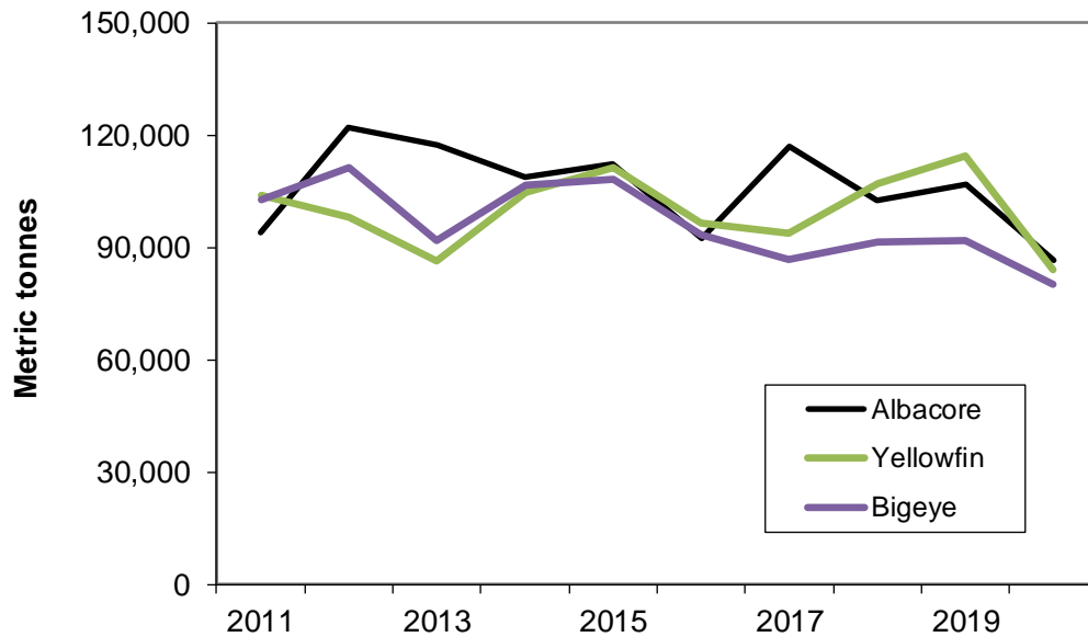
Figure 116. Reported longline tuna catches in the Pacific Ocean
