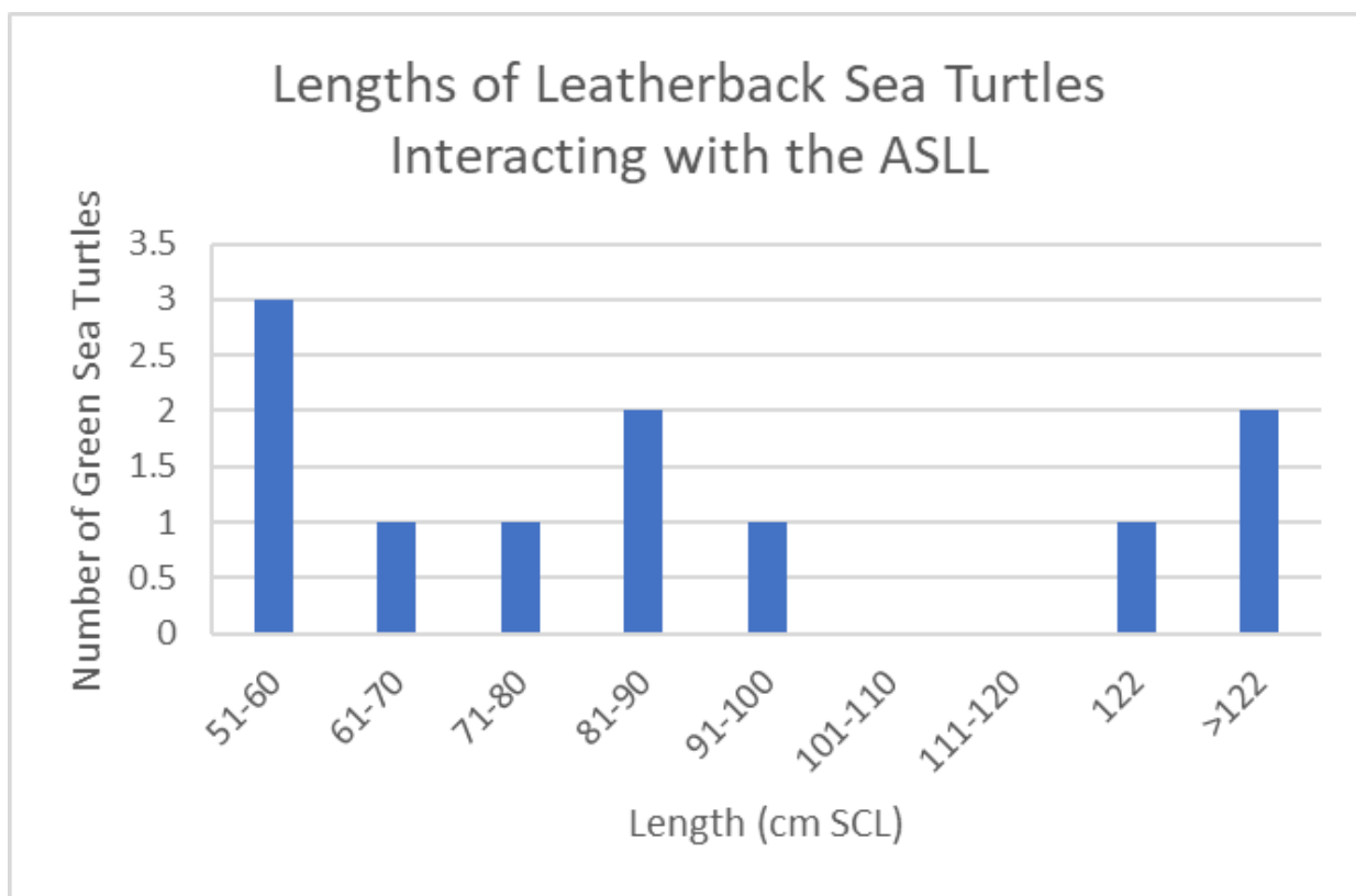
Figure 37. Lengths of observed leatherback sea turtles interacting with the ASLL fishery from 2011 to 2019.
