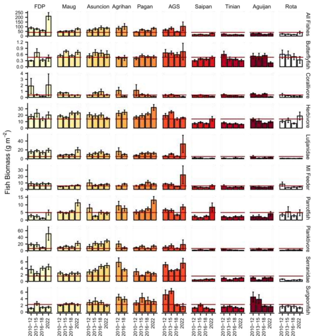
Figure 4. Mean fish biomass (g/m 2 ± SEM) of CNMI functional, taxonomic, and trophic groups over the years 2010-2022 by island. The group ‘Serranidae’ excludes planktivorous members of that family (i.e., anthias, which can be hyper-abundant in some regions). Similarly, the bumphead parrotfish, Bolbometopon muricatum , has been excluded from the corallivore group. The group ‘MI Feeder’ consists of fishes that primarily feed on mobile invertebrates, ‘Butterflyfish’ are non-planktivorous butterflyfish species, and ‘Surgeonfish’ are mid-large target surgeonfish species. Red horizontal lines are the region-wide mean estimates for reference
