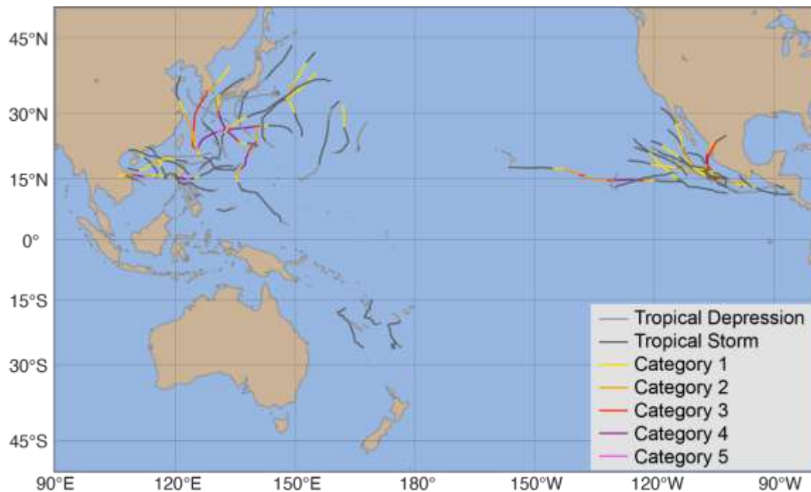
Figure 22. 2022 Pacific basin tropical cyclone tracks
