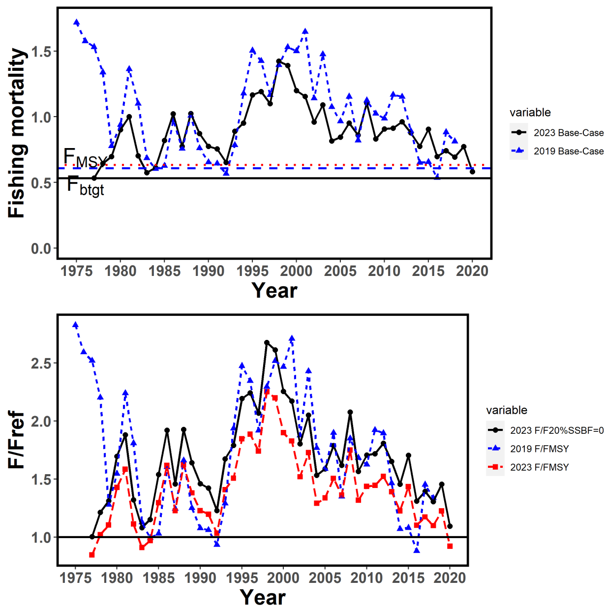
Figure 37. Comparison of the annual fishing mortality (top) and relative fishing mortality (bottom) for the 2019 and 2023 WCNPO striped marlin base-case models. Black solid is the 2023 base-case F_{20\%SSB(F=0)} values, blue short-dashed is the 2019 base-case F_{MSY} values, and red long-dashed is the 2023 base-case F_{MSY} values.
