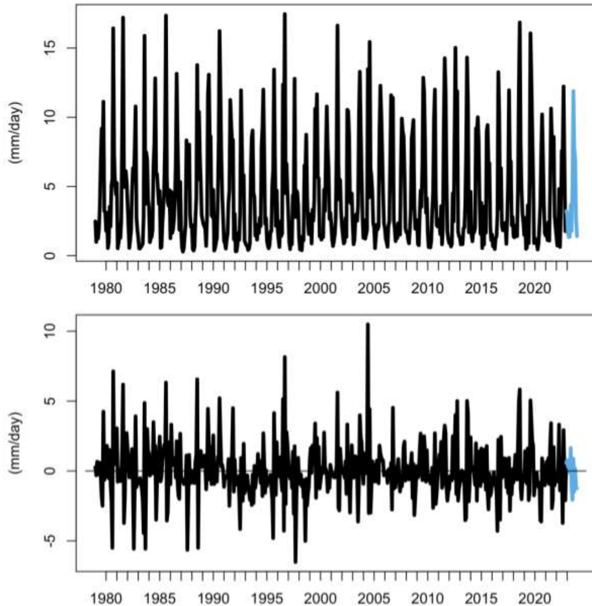
Figure 29. CMAP precipitation (top) and anomaly (bottom) across the Marianas Grid with 2023 values in blue
