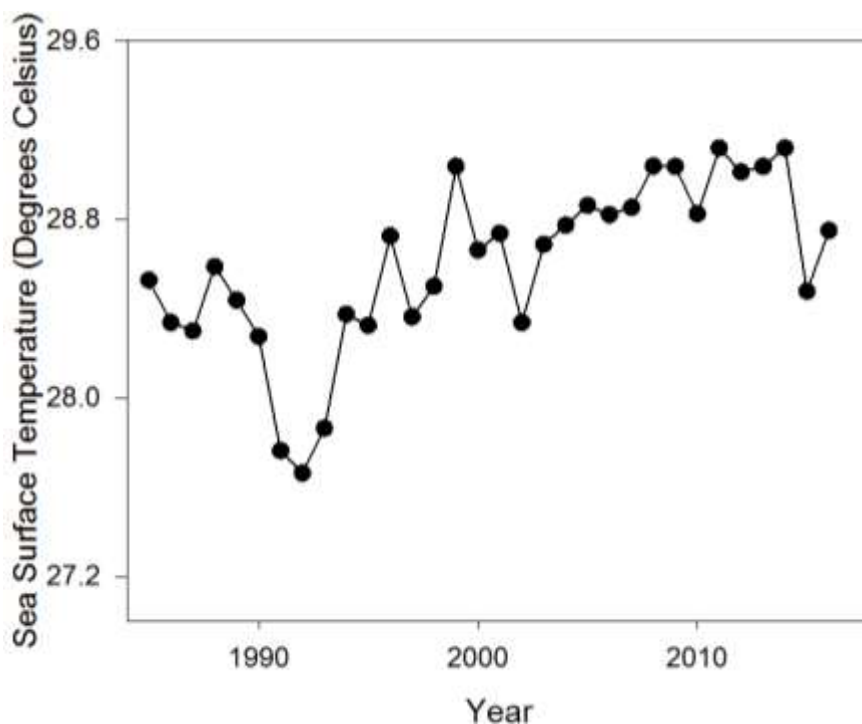
Figure 40. Time series of SST ( ^{\circ}\text{C} ) from 1985-2016 in Guam ( CV = 1.38 )
