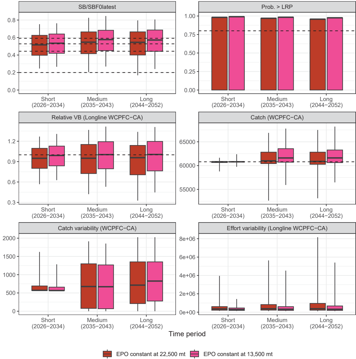
Figure 6: The performance indicators where the constant catch level in the EPO is 22,500 mt and 13,500 mt. A catch-based MP with HCR 1 is used, with \pm 10\% constraint. The whiskers show the 95th percentile range, the box shows the 60th percentile range, and the horizontal line is the median value. The probability of being above LRP is shown as a bar plot.
