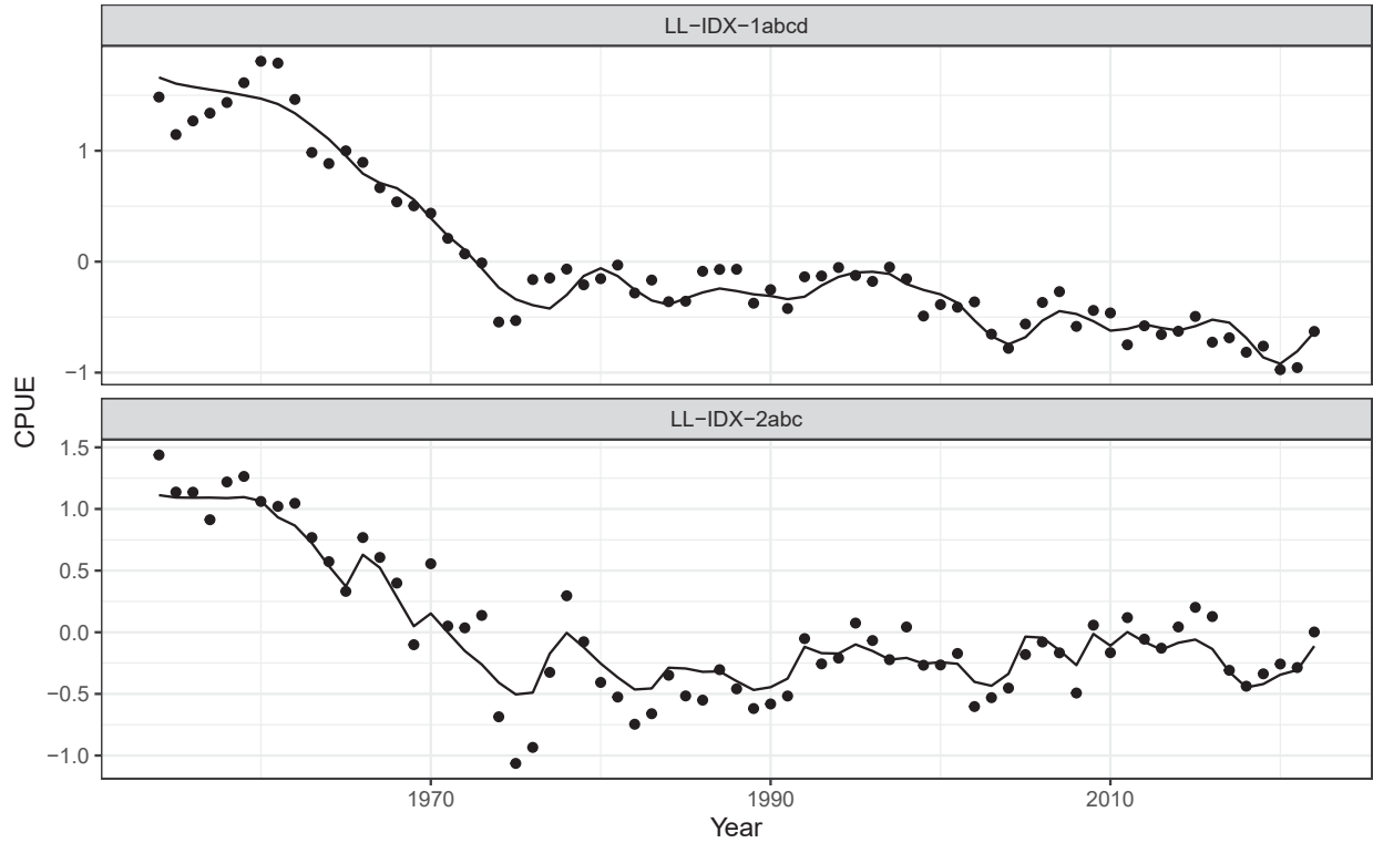
Figure 8: Observed (points) and predicted (lines) CPUE for the index fisheries (top panel is WCPFC-CA, bottom panel is EPO) from the EM for the dry run analysis.
