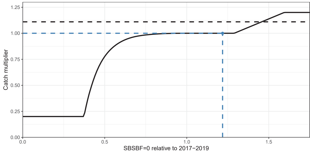
Figure 9: The result from the dry run analyses, using input data up to 2022 and a catch-based MP with HCR 1. The estimated stock status from the EM is used as the input to the HCR (vertical blue dashed line). The horizontal blue dashed line shows the resulting scaler with no constraint. The horizontal black dashed line shows the effective scaler from the previous time period, i.e. the catch level in 2022, relative to the baseline catch level (the average of 2020-2022), to which any constraint would be applied.
