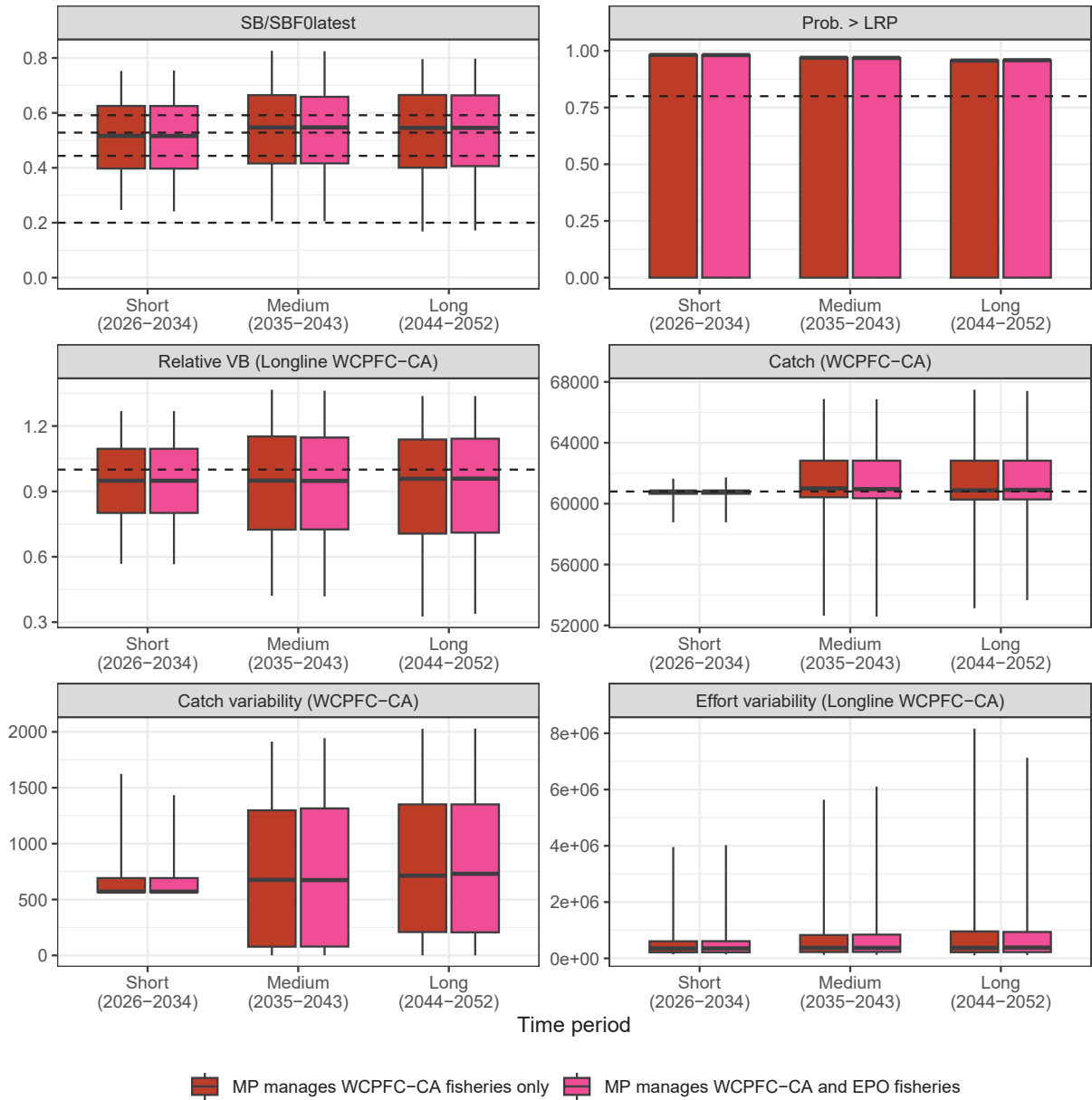
Figure 7: The performance indicators where the EPO fisheries are also managed through the MP, with a baseline of 22,500 mt. A catch-based MP with HCR 1 with \pm 10\% constraint is used. The whiskers show the 95th percentile range, the box shows the 60th percentile range, and the horizontal line is the median value. The probability of being above LRP is shown as a bar plot.
