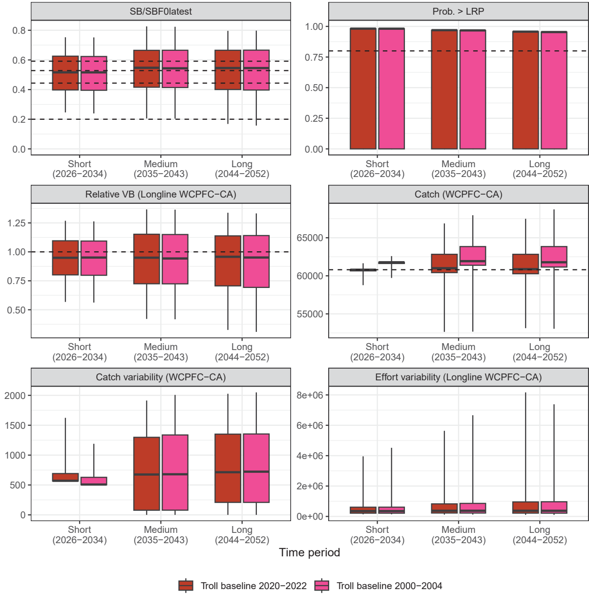
Figure 5: The performance indicators where the HCR baseline for all fisheries in the WCPFC-CA is 2020–2022 catches and when the HCR baseline for the troll fisheries in the WCPFC-CA is 2000–2004 catch (others at 2020–2022 catches). A catch-based MP with HCR 1 is used, with \pm 10\% constraint. The whiskers show the 95th percentile range, the box shows the 60th percentile range, and the horizontal line is the median value. The probability of being above LRP is shown as a bar plot.
