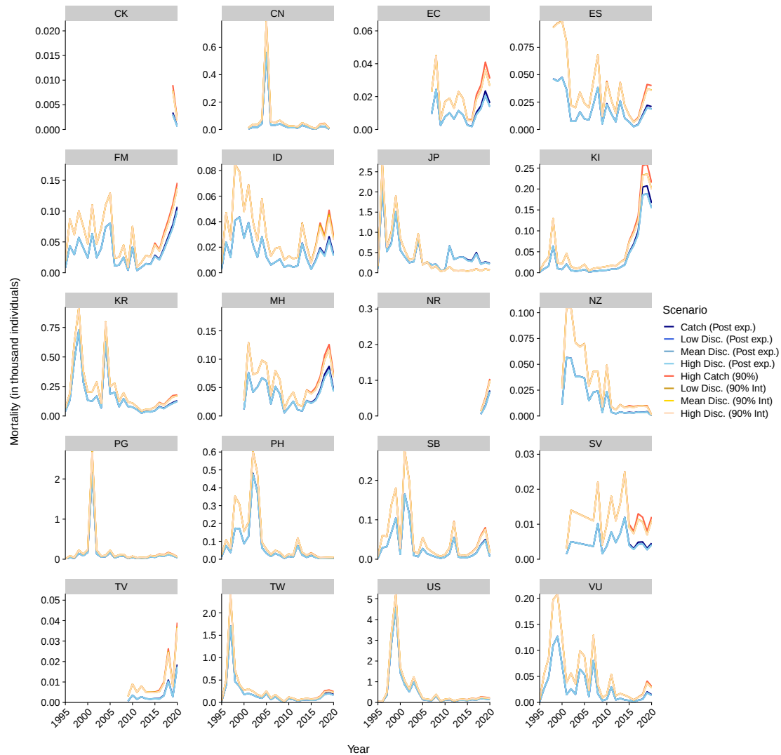
Figure 13: Predicted total fishing related mortality from purse-seine fisheries by flag, including 85% post release mortality for live-discarded oceanic whitetip shark. Interactions refer to the posterior median (50%) and 90 th percentile (90%) of the predicted catch from the observer catch rate model. Low, median and high discard scenarios refer to the 25%, 50% (median) and 75% discard estimates.
