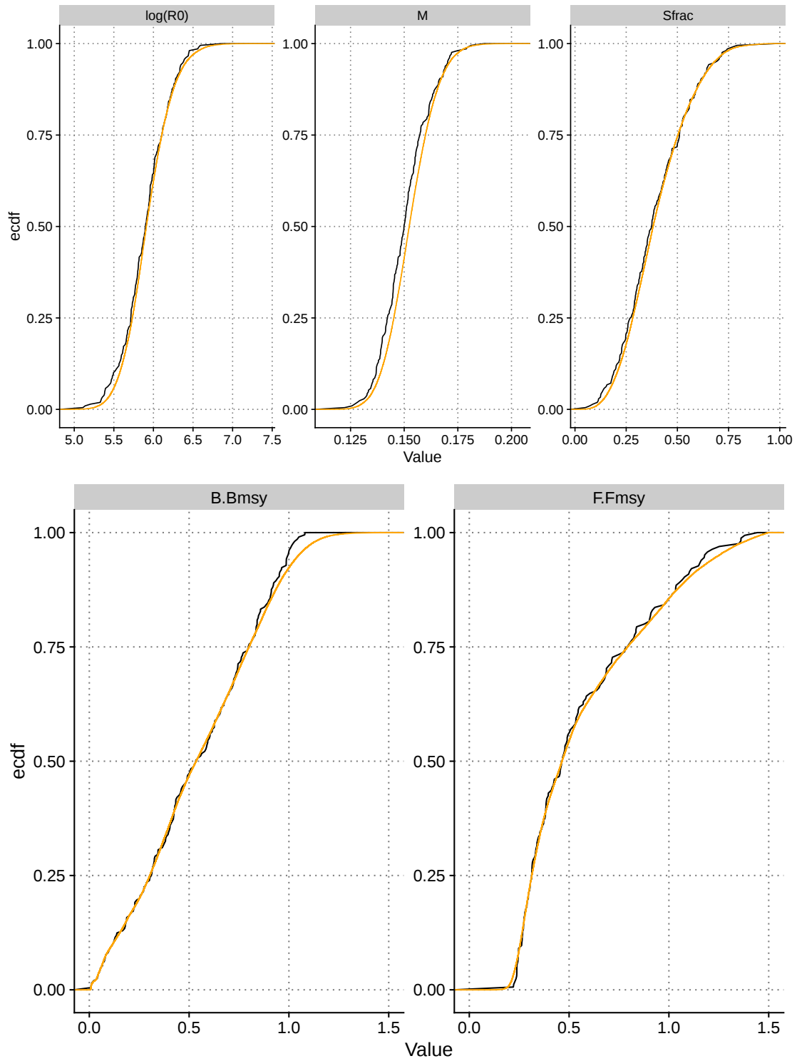
Figure 34: Comparison of the joint simulation-based calibration posterior (orange) to the cumulative distribution of prior draws that were used to simulate the SBC datasets, for model parameters (top panel) and derived management quantities (bottom panel).
